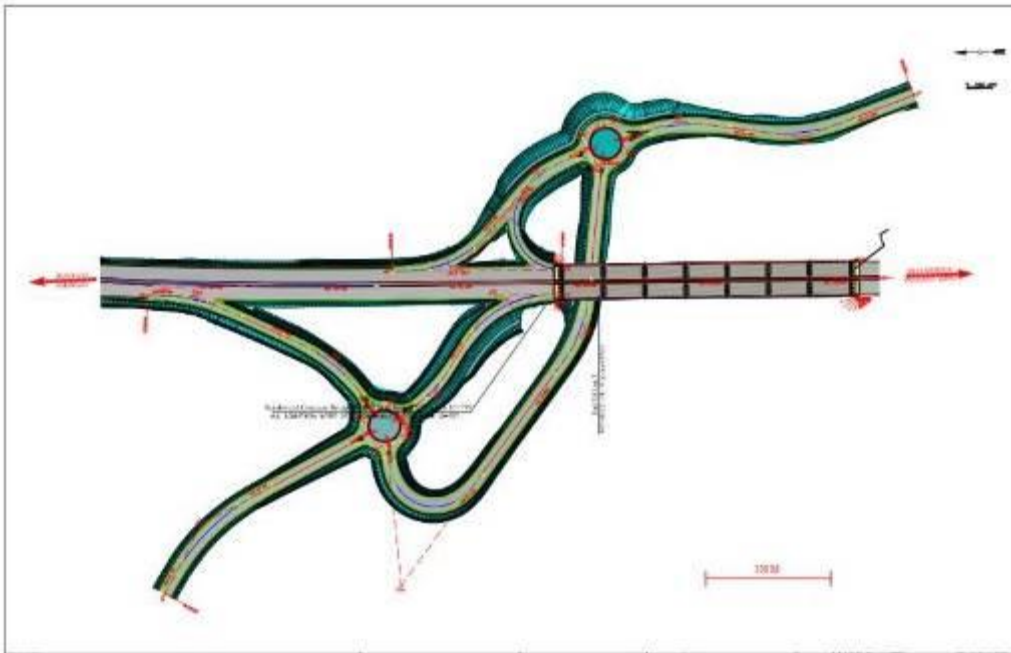
Figure 4.4.7. Red Bridge interchange, 10+705
