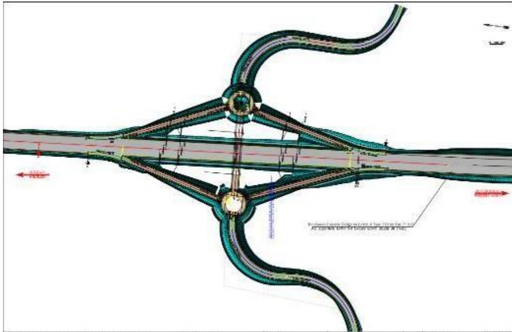
Figure 4.4.3. Azizkendi Interchange 17+305
