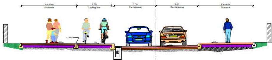
10 SECTION ANA CHAVES BAY (Ch 5+280 - 5+800) SCALE 1:50
