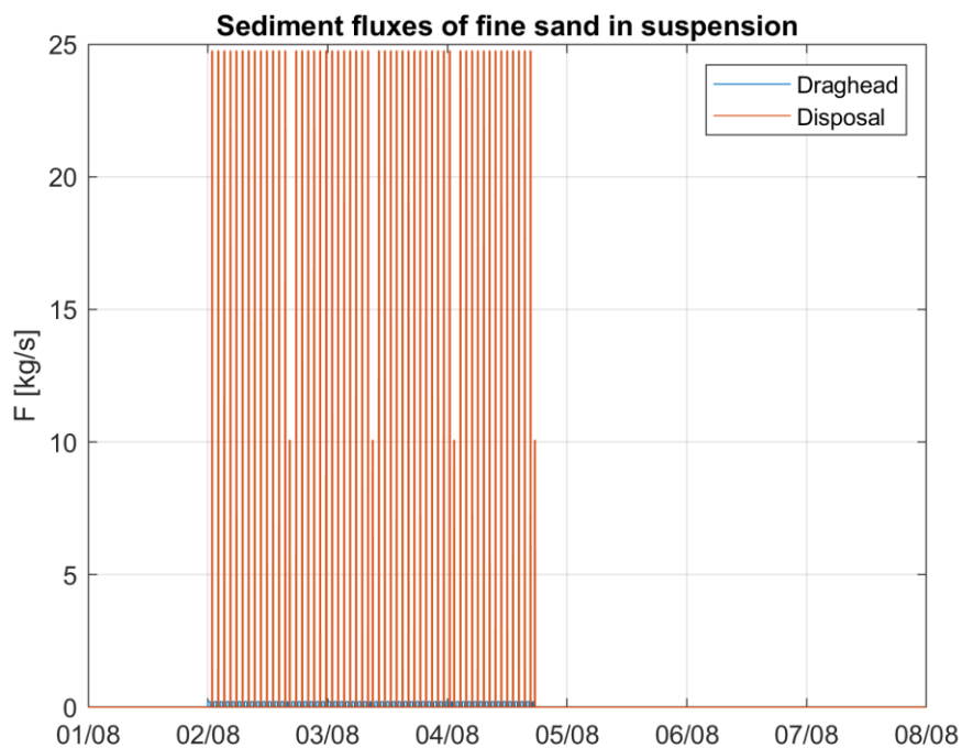
Figure Annex A-10 Time series of the implemented source of fine sand [ \text{kg/s} ] as a result dredging trenches at trench section 2 for the power cables and disposing dredged material at a temporary disposal site 3.
