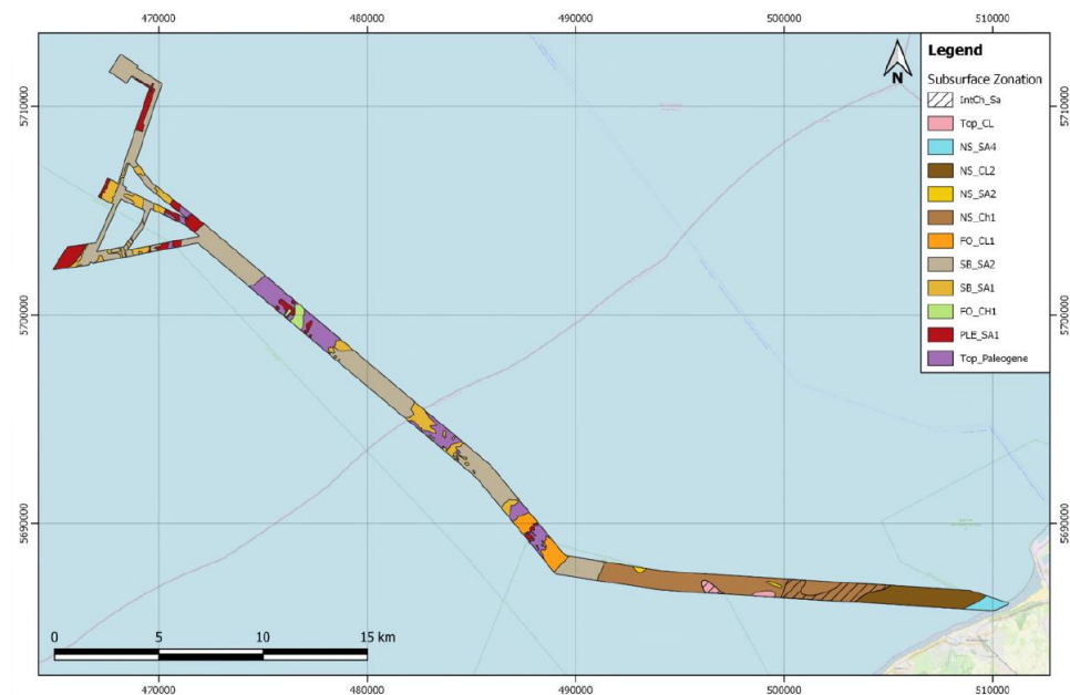
Figure 2-9 Subsurface sediment unitization, adapted from Cathie draft report (2021) along the power cable track. Grey zones = sandy regime, purple and orange zones = stiff clayey regime, brown zones = muddy/silty regime.
