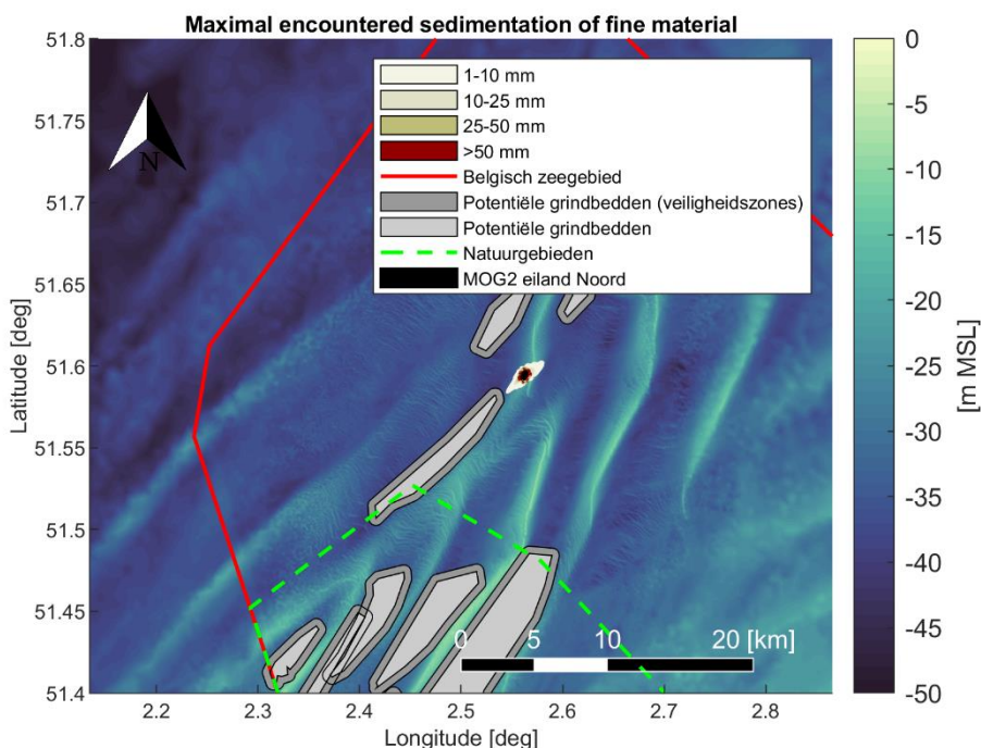
Figure 4-6 Maximal encountered sedimentation [mm] of fine material (< 250 [μm]) during the simulation period. Scenario 2: pre-dredging scour holes and creation of sand plateau at the island location Noord.
