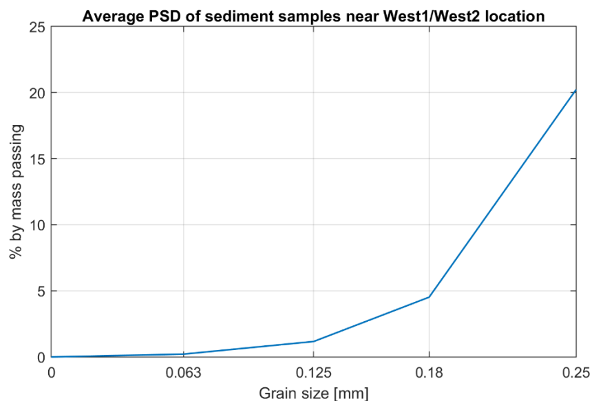
Figure 2-14 Average particle size distribution (PSD) of vibrocore locations (Mathys et al., 2009) within the green circle of Figure 4-4.
