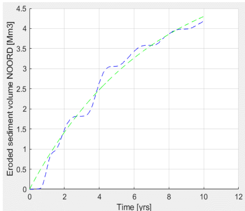
Figure 3-4 Example of total simulated eroded sediment volume due to the implementation of the MOG2 island at the Noord location (blue line) provided by Svašek. The green line shows a fit through the original dataset.
