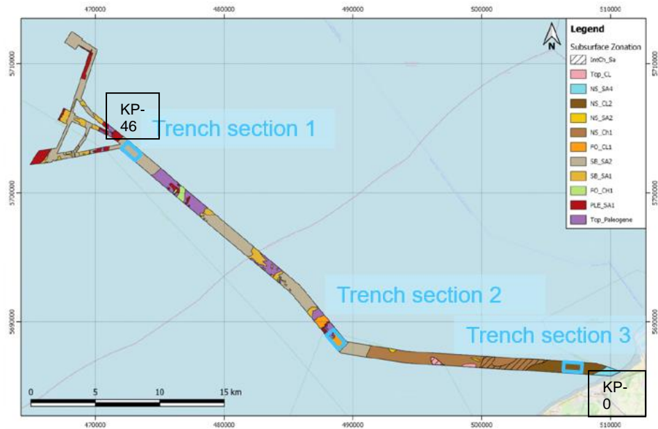
Figure 3-2 Subsurface sediment unitization, adapted from Cathie draft report (2021) along the power cable track and locations of simulated trench sections.
