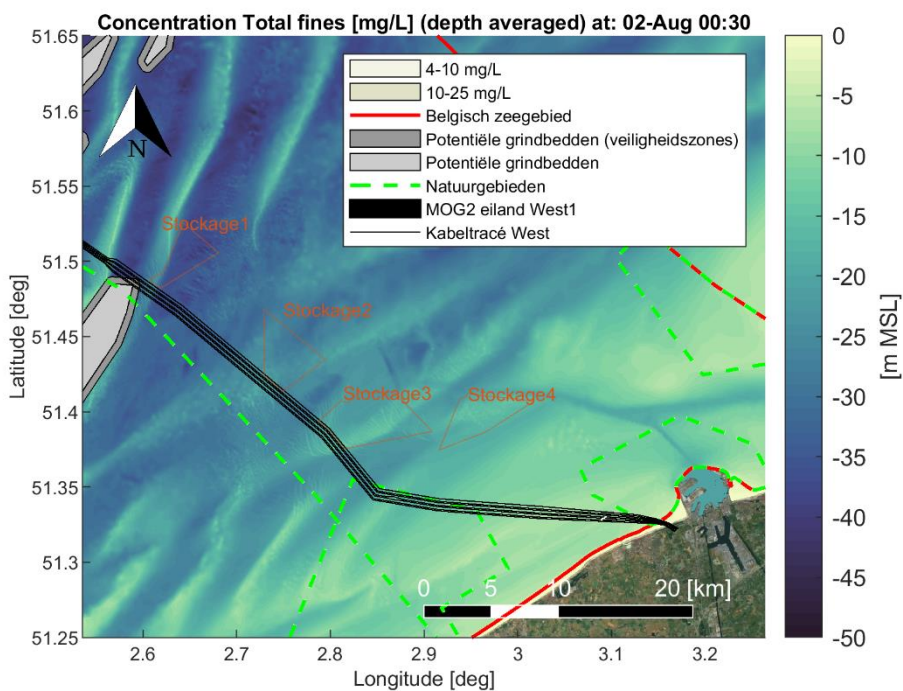
Figure Annex B-2 Map showing encountered depth averaged sediment concentration [mg/L] of fine material (< 250 [µm]) during a time instant of the simulation period. Scenario: Dredging cable trenches (trench1 section) and disposal at a temporary disposal site (Stockage3). Satellite background image credit: "OpenMapTiles.org".
