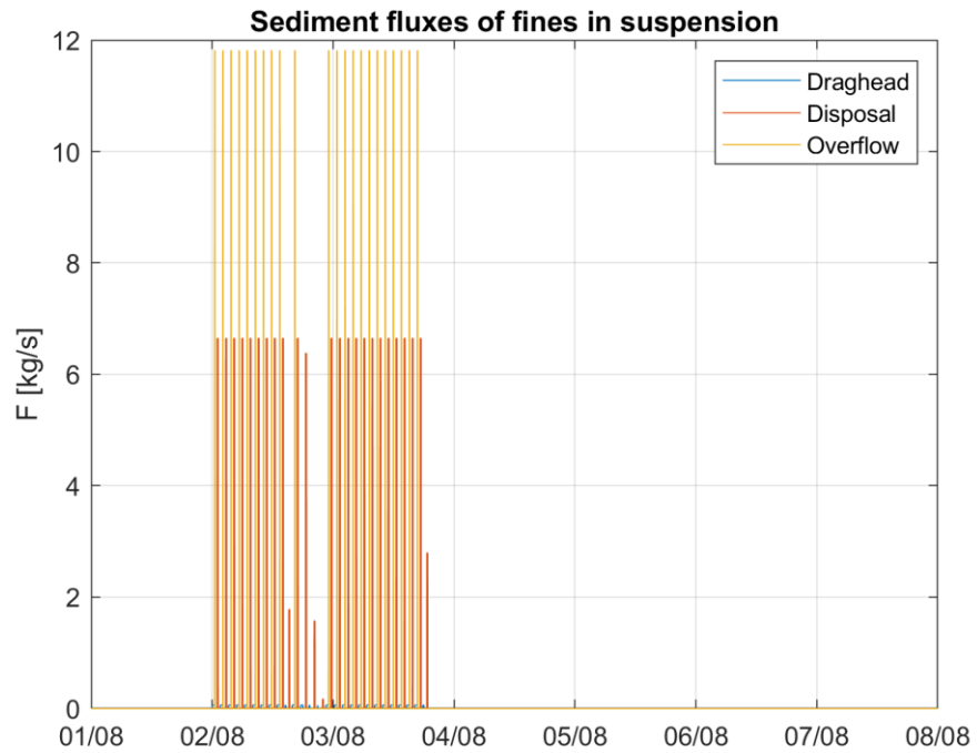
Figure 7-1 Time series of the implemented source of fines ( d_p < 63 \mu\text{m} ) [kg/s] as a result of dredging works related to the levelling of sand ridge crests at the West 1 location.
