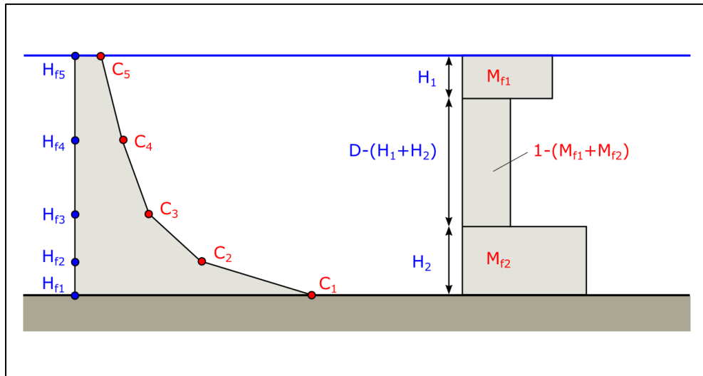
Figure 2-17 Two types of representing vertical distributions. Left: Flag type F1 based on a sigma distribution over the vertical and the concentration profile, Right: Flag type F2 based on representing the heights and mass fractions of two blocks near the surface and near the bed, in between the rest of the material is distributed.
