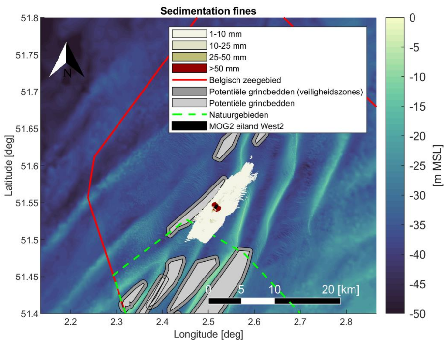
Figure 4-27 Maximal encountered sedimentation [mm] of fine material (< 250 [μm]) during the simulation period. Scenario: Plume generation and deposition as a result of natural erosion in one year time after West 2 island construction, after four year case.
