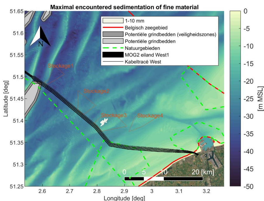
Figure 4-16 Maximal sedimentation [mm] of fine material (< 250 \mu\text{m} ) during the simulation period. Scenario: Dredging cable trenches (trench 2 section) and disposal at a temporary disposal site (Stockage3). Satellite background image credit: "OpenMapTiles.org".
