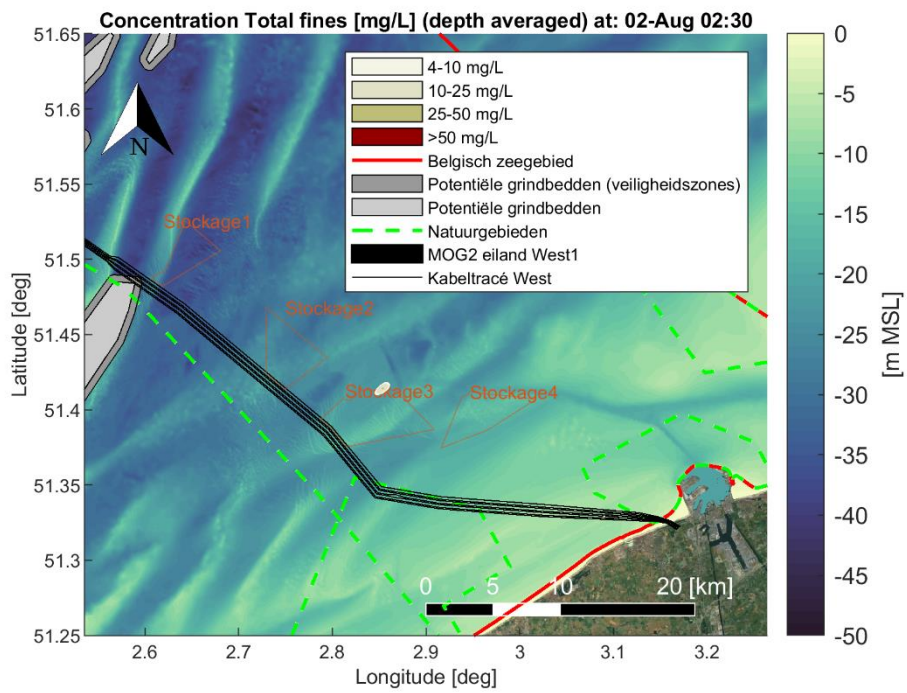
Figure Annex B-6 Map showing encountered depth averaged sediment concentration [mg/L] of fine material (< 250 [µm]) during a time instant of the simulation period. Scenario: Dredging cable trenches (trench1 section) and disposal at a temporary disposal site (Stockage3). Satellite background image credit: "OpenMapTiles.org".
