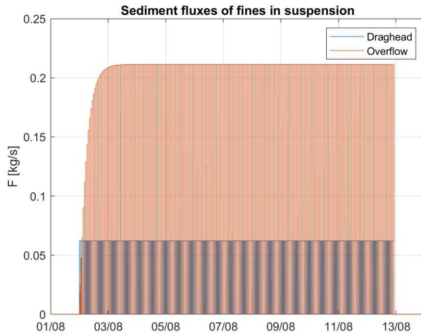
Figure Annex A-1 Time series of the implemented source of fines ( d_p < 63 \text{ mm} ) [ \text{kg/s} ] as a result of pre-dredging scour holes and ridges and filling the island ring with dredged sand through pipes, leading to overflow from the island ring at the West 1 location.
