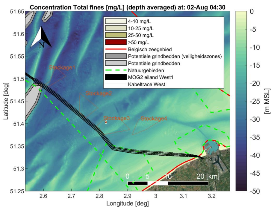
Figure Annex B-10 Map showing encountered depth averaged sediment concentration [mg/L] of fine material (< 250 [µm]) during a time instant of the simulation period. Scenario: Dredging cable trenches (trench1 section) and disposal at a temporary disposal site (Stockage3). Satellite background image credit: "OpenMapTiles.org".
