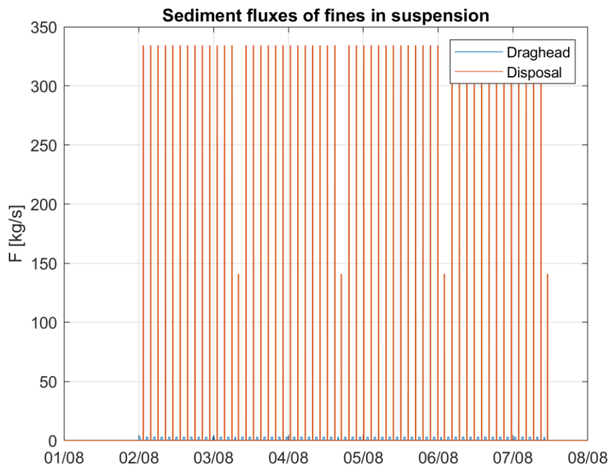
Figure Annex A-11 Time series of the implemented source of fines ( d_p < 63 \mu\text{m} ) [ \text{kg/s} ] as a result dredging trenches at trench section 3 for the power cables and disposing dredged material at a temporary disposal site 3.
