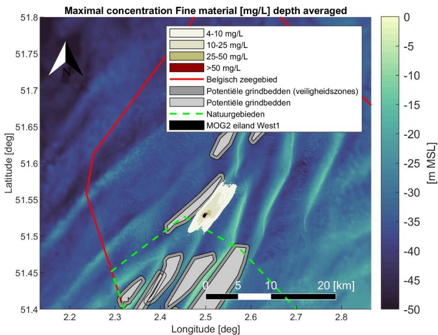
Figure 4-22 Maximal depth averaged sediment concentration [mg/L] of fine material (< 250 [μm]) during the simulation period. Scenario: : Plume generation and deposition as a result of natural erosion in one year time after West 1 island construction, after one year case.
