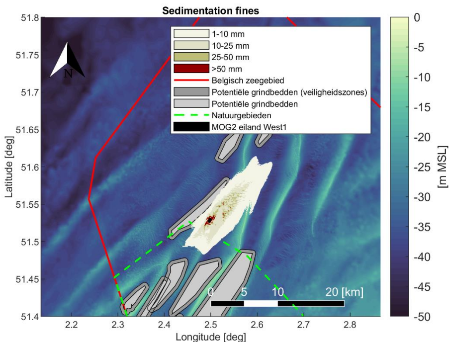
Figure 4-33 Maximal encountered sedimentation [mm] of fine material (< 250 µm) during the simulation period. Scenario: Plume generation and deposition as a result of natural erosion in one year time after West 1 island construction, after one year case including pre-scour design.
