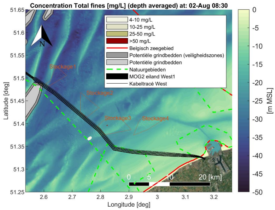
Figure Annex B-18 Map showing encountered depth averaged sediment concentration [mg/L] of fine material (< 250 [μm]) during a time instant of the simulation period. Scenario: Dredging cable trenches (trench1 section) and disposal at a temporary disposal site (Stockage3). Satellite background image credit: "OpenMapTiles.org".
