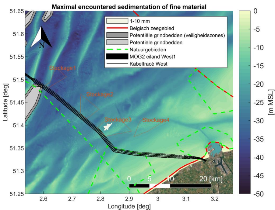
Figure 4-18 Maximal sedimentation [mm] of fine material (< 250 [μm]) during the simulation period. Scenario: Dredging cable trenches (trench 3 section) and disposal at a temporary disposal site (Stockage3). Satellite background image credit: "OpenMapTiles.org".
