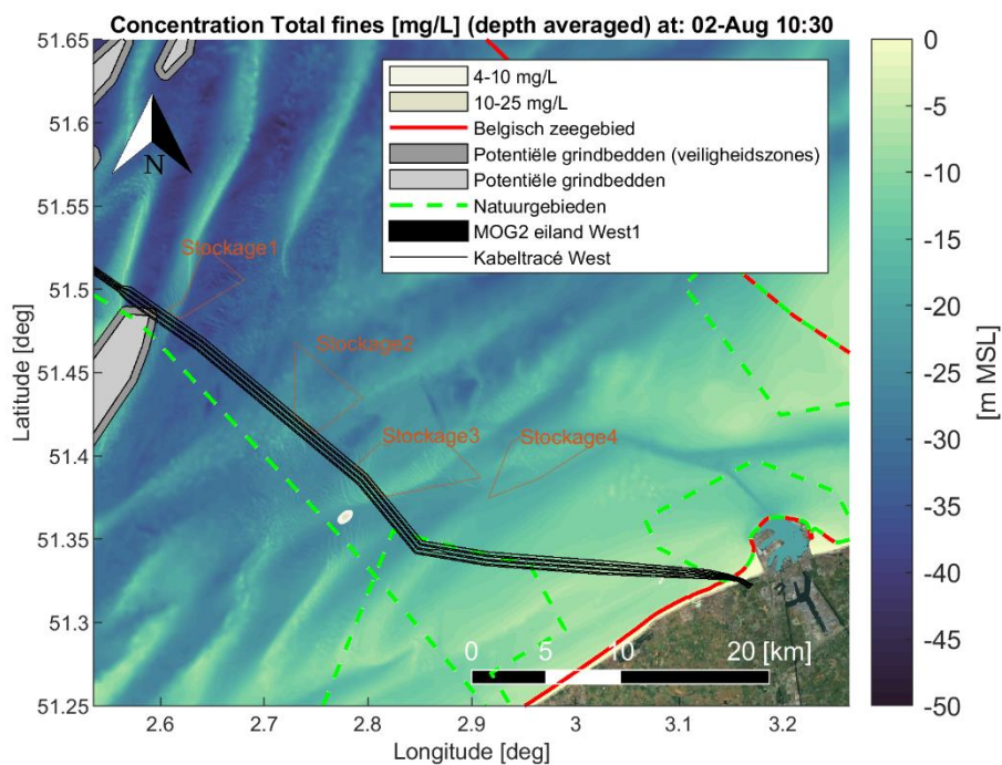
Figure Annex B-22 Map showing encountered depth averaged sediment concentration [mg/L] of fine material (< 250 [µm]) during a time instant of the simulation period. Scenario: Dredging cable trenches (trench1 section) and disposal at a temporary disposal site (Stockage3). Satellite background image credit: "OpenMapTiles.org".
