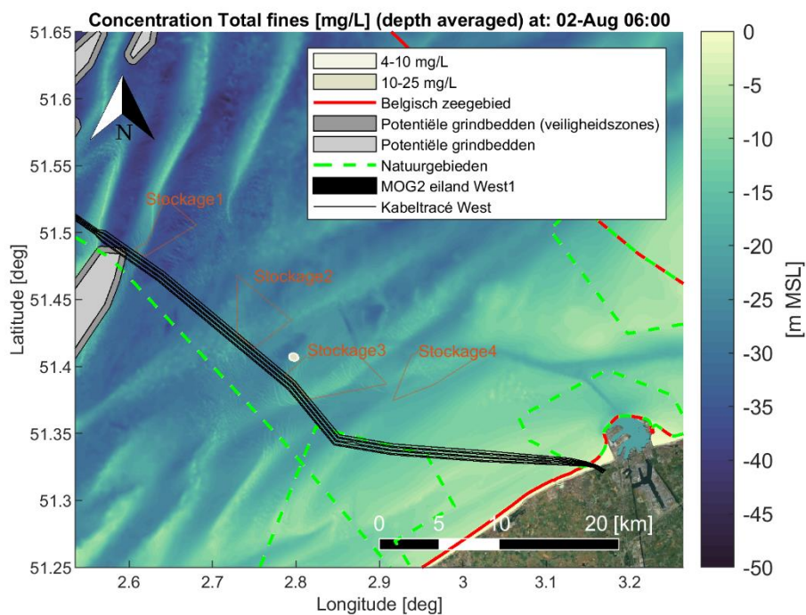
Figure Annex B-13 Map showing encountered depth averaged sediment concentration [mg/L] of fine material (< 250 [µm]) during a time instant of the simulation period. Scenario: Dredging cable trenches (trench1 section) and disposal at a temporary disposal site (Stockage3). Satellite background image credit: "OpenMapTiles.org".
