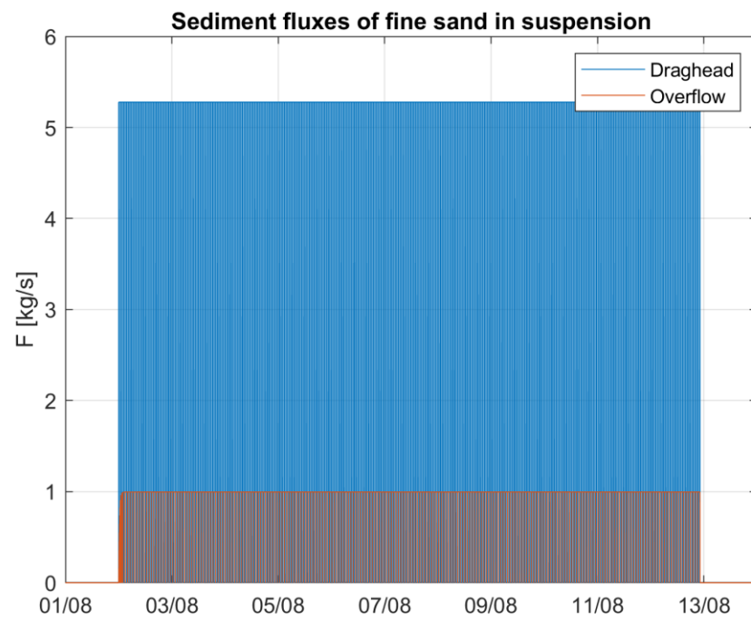
Figure Annex A-6 Time series of the implemented source of fine sand [kg/s] as a result of pre-dredging scour holes and ridges and filling the island ring with dredged sand through pipes, leading to overflow from the island ring at the Noord location.
