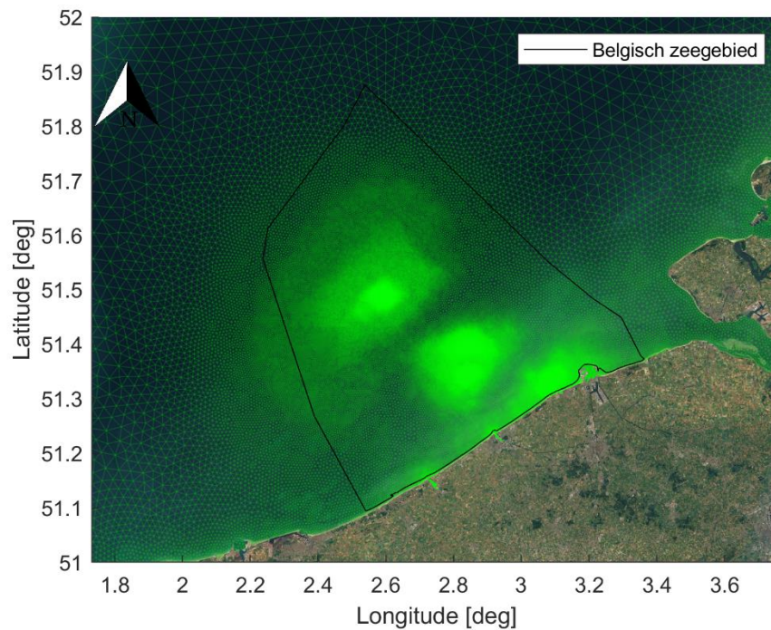
Figure 2-2 Computational mesh, zoom-in around the Belgian part of the North sea. Satellite background image credit: "OpenMapTiles.org".
