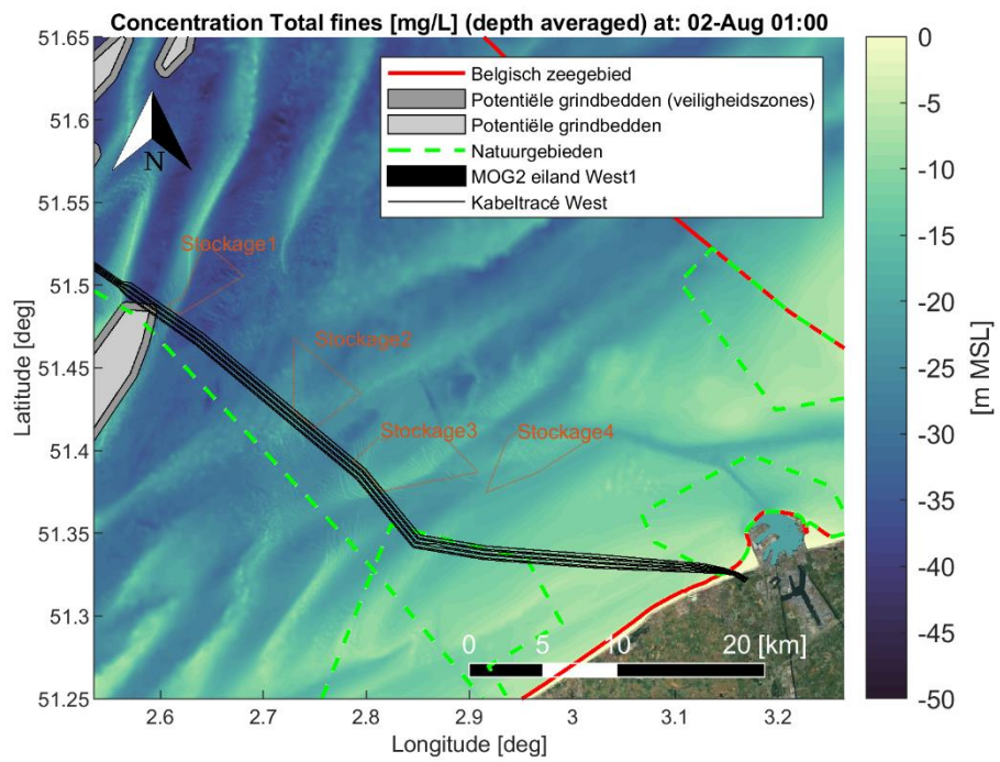
Figure Annex B-3 Map showing encountered depth averaged sediment concentration [mg/L] of fine material (< 250 [μm]) during a time instant of the simulation period. Scenario: Dredging cable trenches (trench1 section) and disposal at a temporary disposal site (Stockage3). Satellite background image credit: "OpenMapTiles.org".
