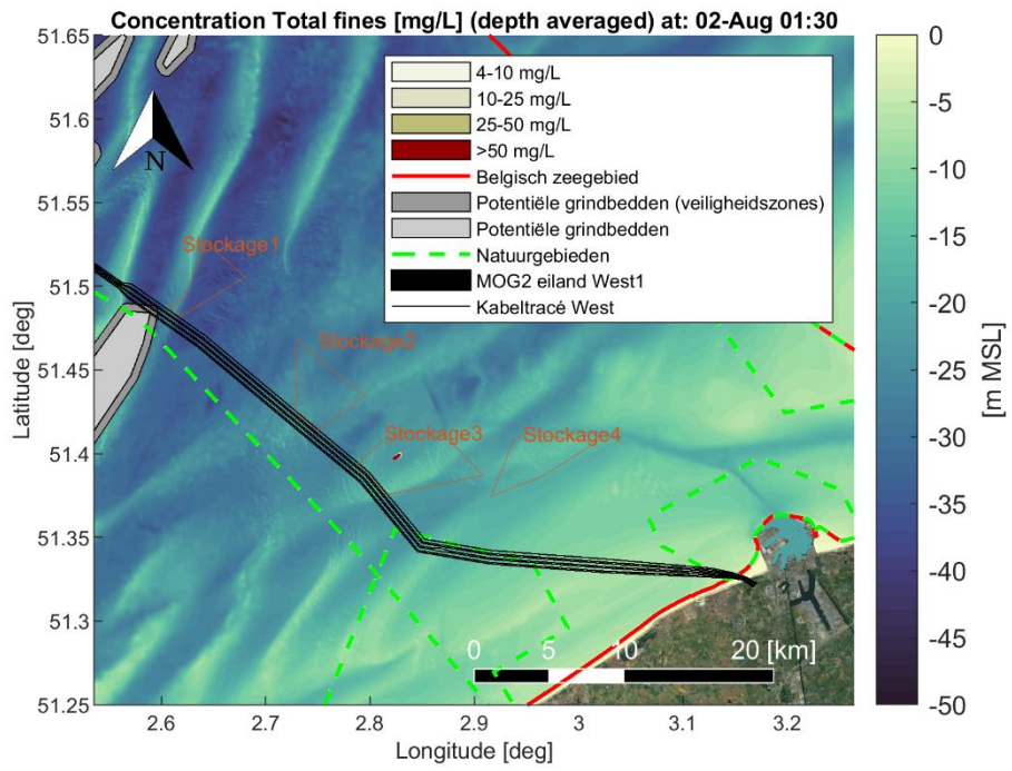
Figure Annex B-4 Map showing encountered depth averaged sediment concentration [mg/L] of fine material (< 250 [µm]) during a time instant of the simulation period. Scenario: Dredging cable trenches (trench1 section) and disposal at a temporary disposal site (Stockage3). Satellite background image credit: "OpenMapTiles.org".
