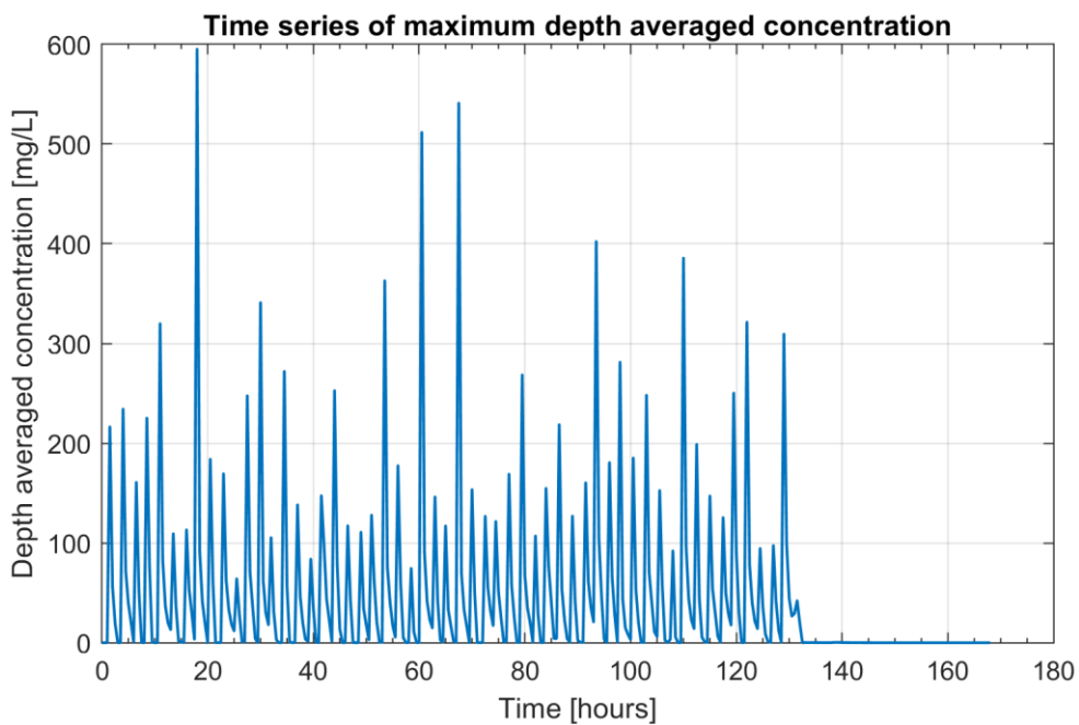
Figure 4-19 Time series of maximal sediment concentration [mg/L] of fine sediment at the temporary disposal site 3, using half-hourly model output.
