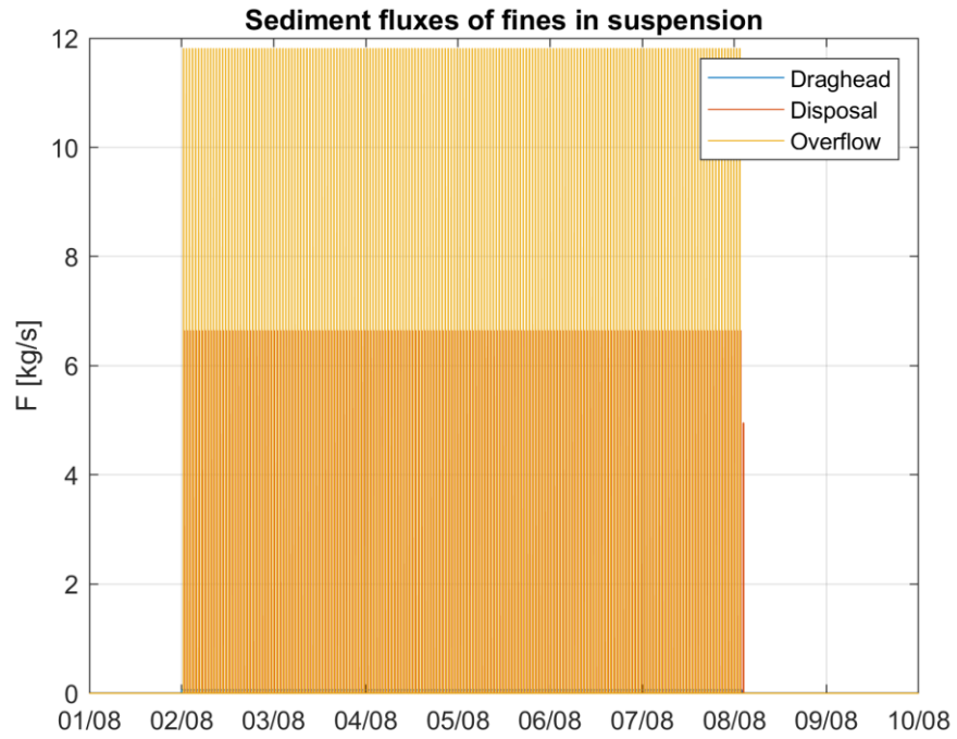
Figure 7-3 Time series of the implemented source of fines ( d_p < 63 \mu\text{m} ) [ \text{kg/s} ] as a result of pre-dredging scour holes and ridges and disposing dredged material at the island location at the West 2 location.
