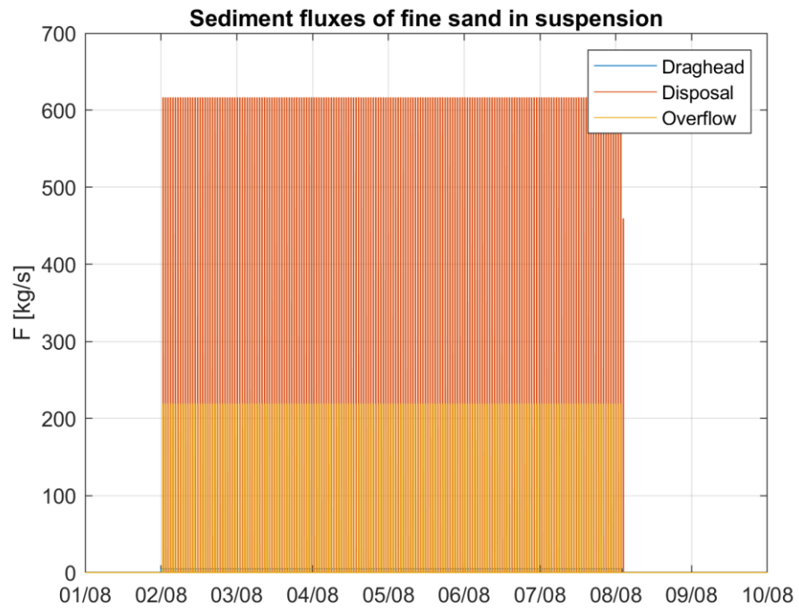
Figure 7-4 Time series of the implemented source of fine sand [kg/s] as a result of pre-dredging l scour holes and ridges and disposing dredged material at the island location at the West 2 location.
