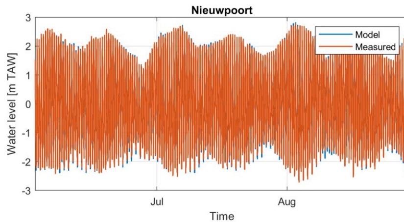
Figure 2-6 Timeseries of modelled and measured water level [m MSL] from 02-0-2019 till 30-08-2019 at the Nieuwpoort measurement station.
