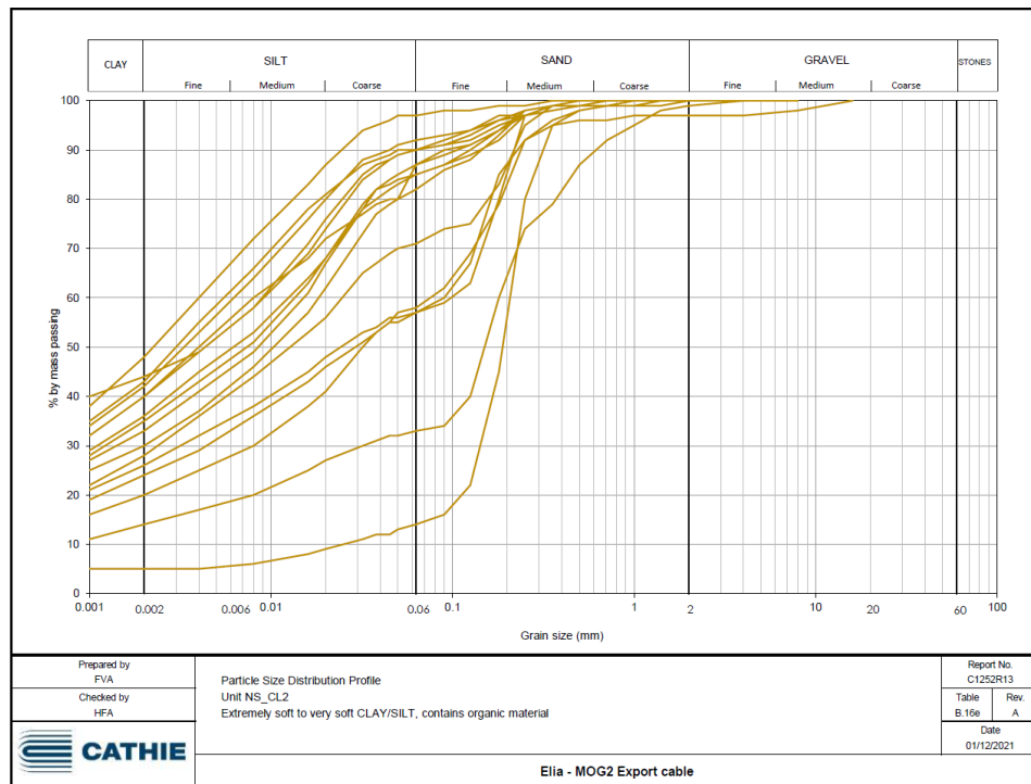
Figure 2-12 Particle size distribution profile of unit NS_CL2 (extremely soft to very soft clay/silt, contains organic material), adapted from Cathie draft report (2021)
