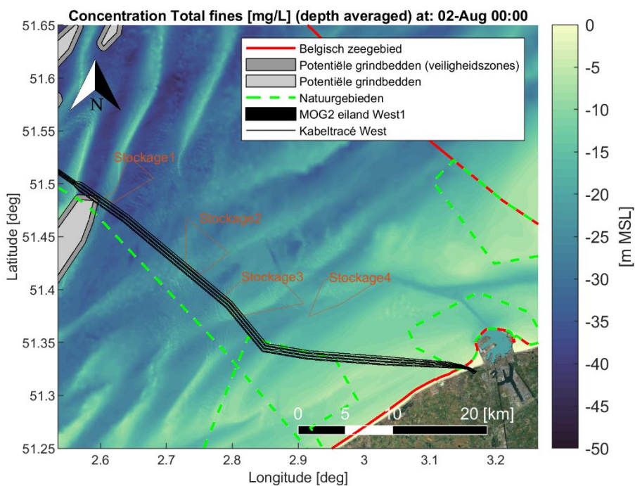
Figure Annex B-1 Map showing encountered depth averaged sediment concentration [mg/L] of fine material (< 250 [µm]) during a time instant of the simulation period. Scenario: Dredging cable trenches (trench1 section) and disposal at a temporary disposal site (Stockage3). Satellite background image credit: "OpenMapTiles.org".
