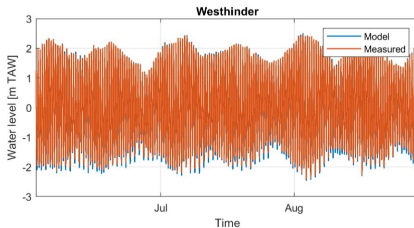
Figure 2-7 Timeseries of modelled and measured water level [m MSL] from 02-0-2019 till 30-08-2019 at the Westhinder measurement station.
