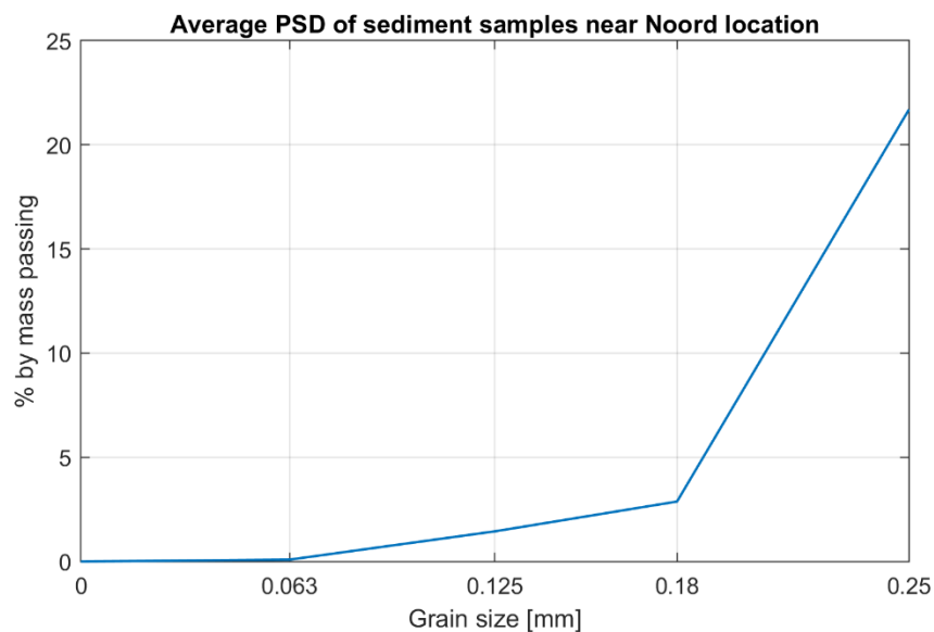
Figure 2-15 Average particle size distribution (PSD) of vibrocore locations (Mathys et al., 2009) within the orange circle of Figure 4-4.
