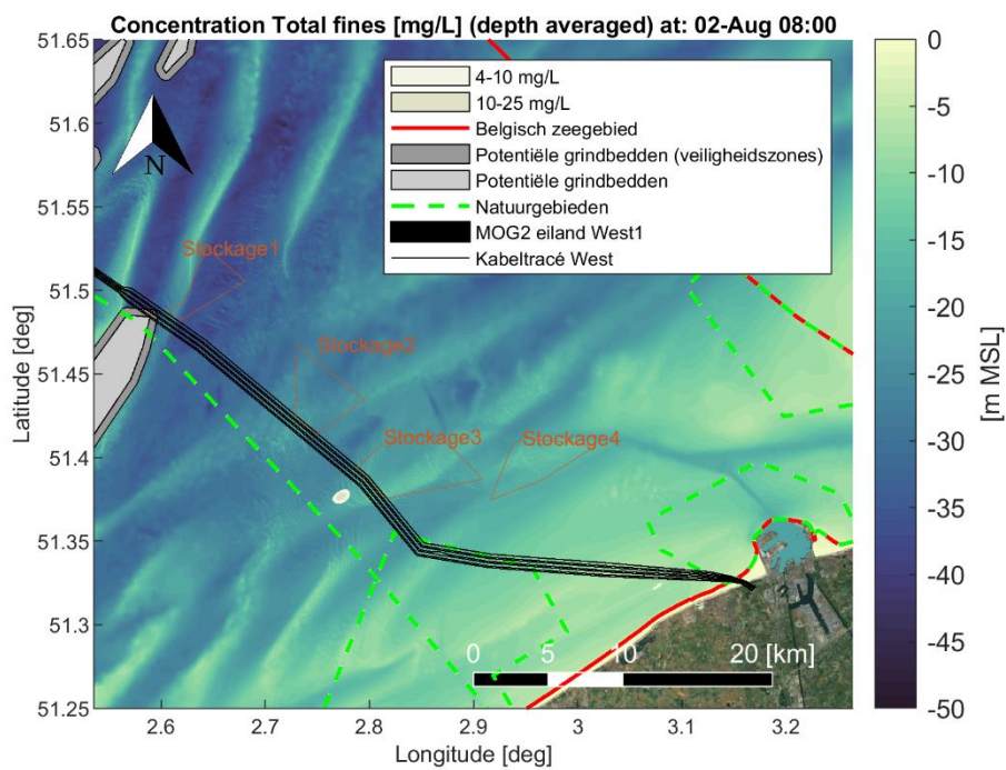
Figure Annex B-17 Map showing encountered depth averaged sediment concentration [mg/L] of fine material (< 250 [µm]) during a time instant of the simulation period. Scenario: Dredging cable trenches (trench1 section) and disposal at a temporary disposal site (Stockage3). Satellite background image credit: "OpenMapTiles.org".
