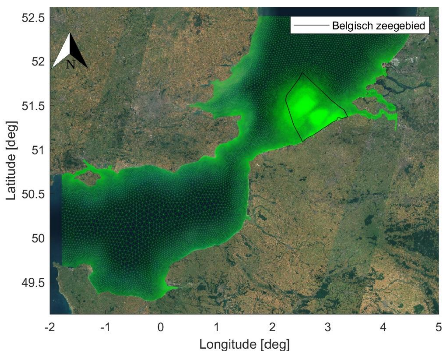
Figure 2-1 Computational mesh. Satellite background image credit: "OpenMapTiles.org".
