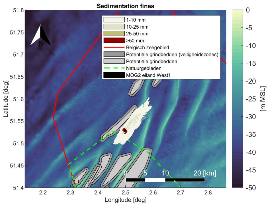
Figure 4-23 Maximal sedimentation [mm] of fine material (< 250 [µm]) during the simulation period. Scenario: : Plume generation and deposition as a result of natural erosion in one year time after West 1 island construction, after four year case.
