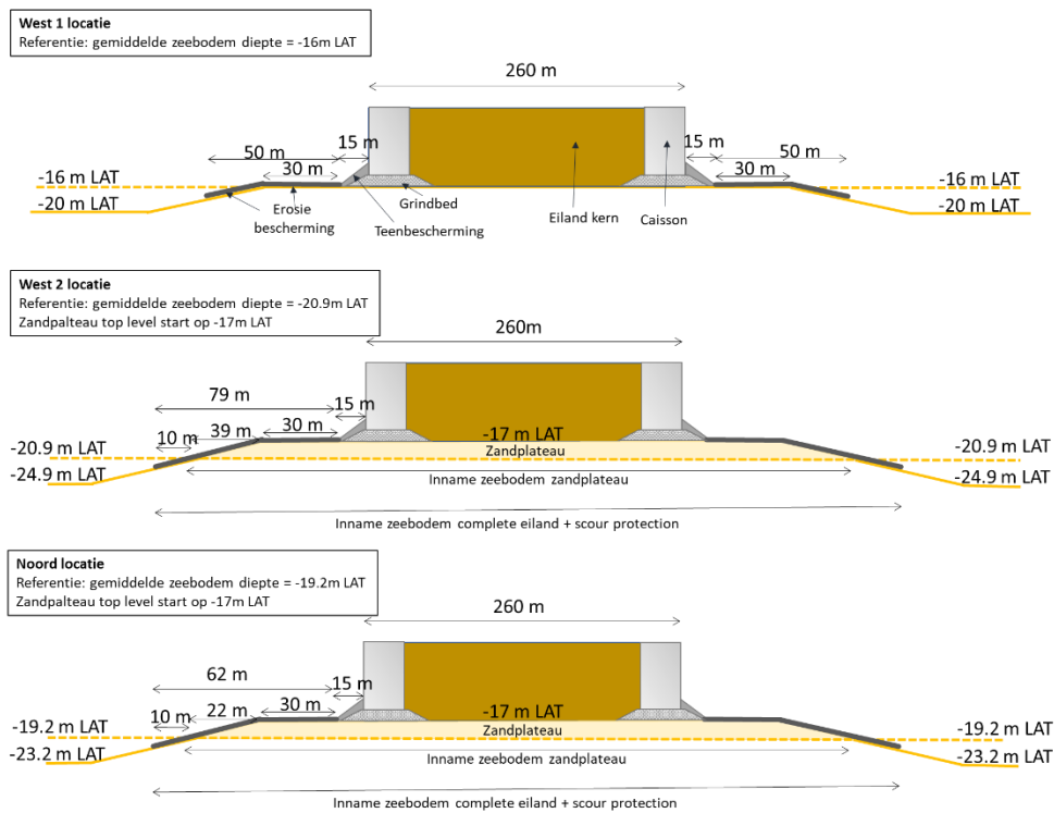
Figure 2-4 Cross-section of proposed island and scour protection dimensions for the West 1 (top), West 2 (mid) and Noord (bottom) location.
