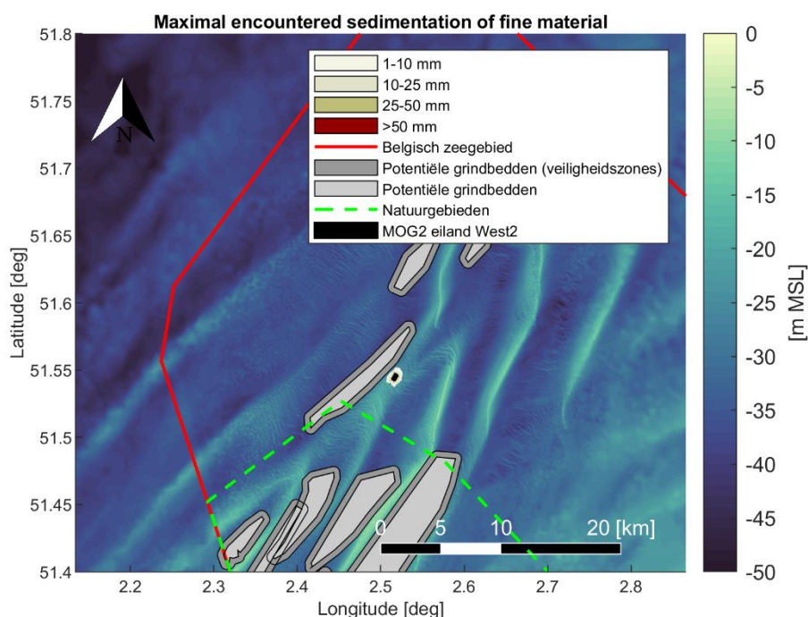
Figure 4-10 Maximal encountered sedimentation [mm] of fine material (< 250 \mu\text{m} ) during the simulation period. Scenario 3: pre-dredging scour holes and filling the West 2 island ring.
