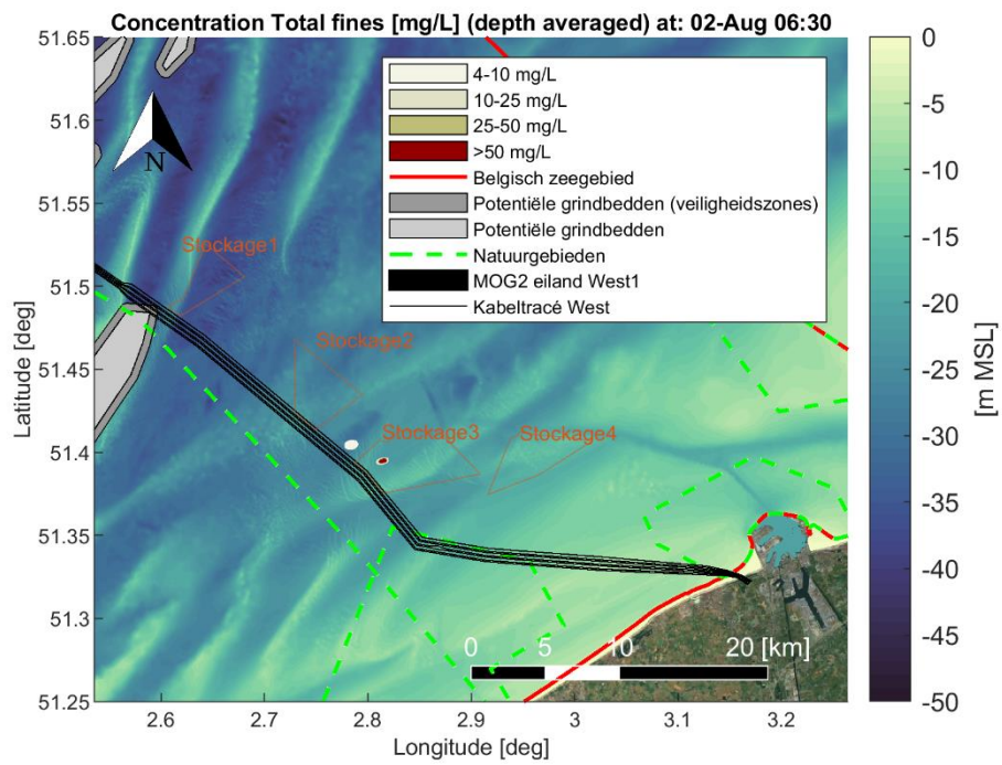
Figure Annex B-14 Map showing encountered depth averaged sediment concentration [mg/L] of fine material (< 250 [μm]) during a time instant of the simulation period. Scenario: Dredging cable trenches (trench1 section) and disposal at a temporary disposal site (Stockage3). Satellite background image credit: "OpenMapTiles.org".
