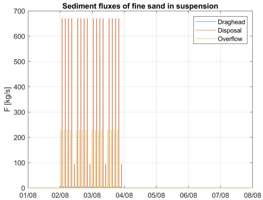
Figure Annex A-8 Timeseries of the implemented source of fine sand [kg/s] as a result dredging trenches at trench section 1 for the power cables and disposing dredged material at a temporary disposal site 3.
