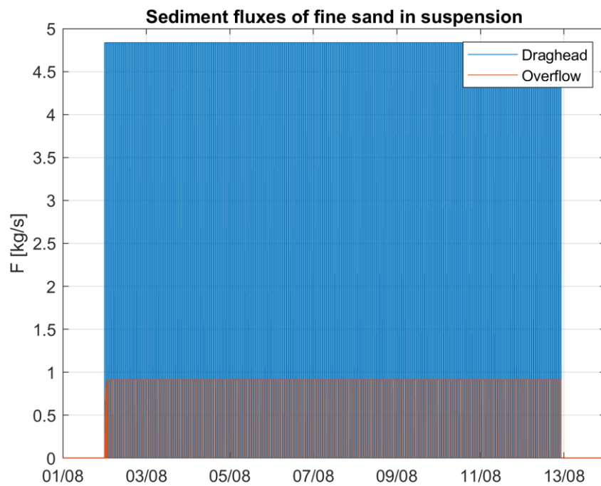
Figure Annex A-4 Time series of the implemented source of fine sand [ \text{kg/s} ] as a result of pre-dredging scour holes and ridges and filling the island ring with dredged sand through pipes, leading to overflow from the island ring at the West 2 location.
