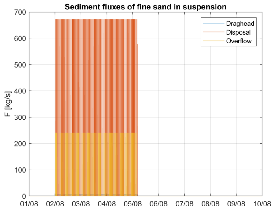
Figure 7-6 Timeseries of the implemented source of fine sand [kg/s] as a result of pre-dredging scour holes and ridges and disposing dredged material at the island location at the Noord location.
