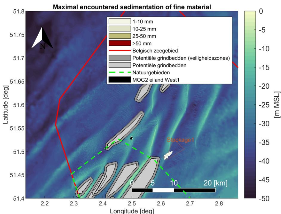
Figure 4-2 Maximal encountered sedimentation [mm] of fine material (< 250 [µm]) during the simulation period. Scenario 1: levelling sand ridges and disposal at a temporary disposal site (island location West 1).
