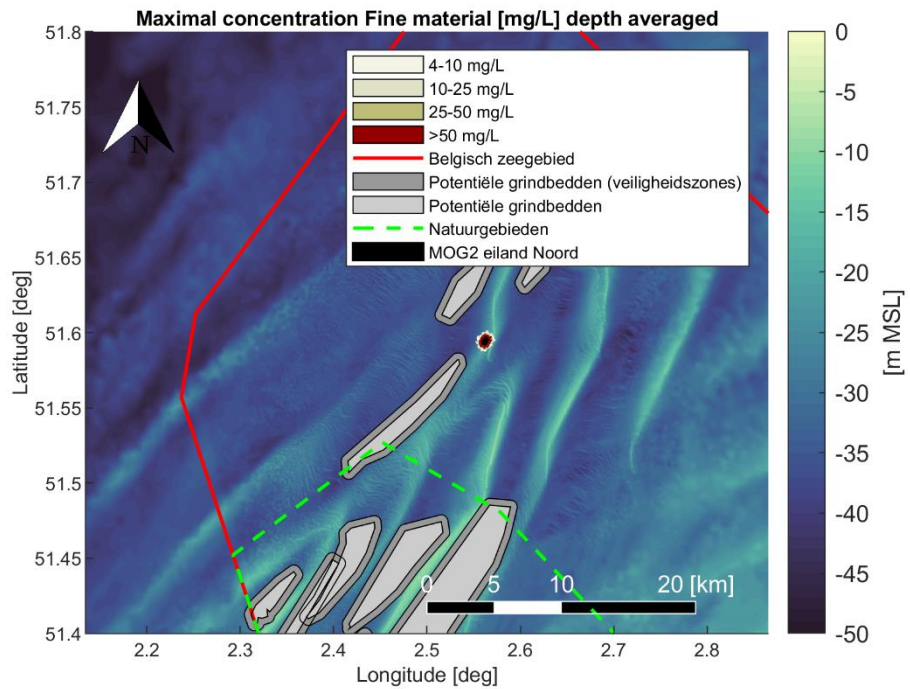
Figure 4-11 Maximal encountered depth averaged sediment concentration [mg/L] of fine material ( < 250 [\mu m] ) during the simulation period. Scenario 3: pre-dredging scour holes and filling the Noord island ring.
