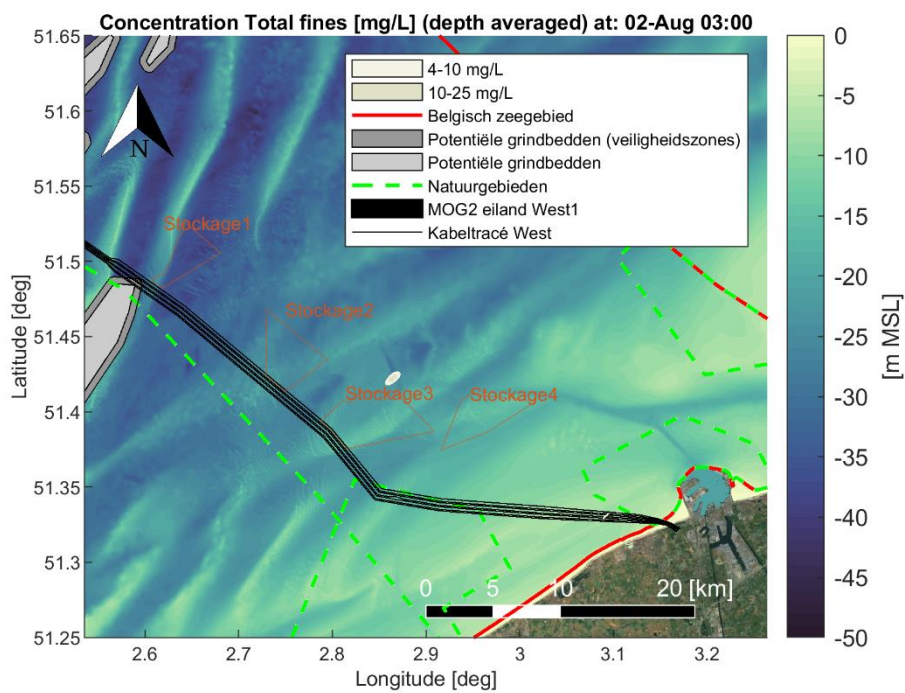
Figure Annex B-7 Map showing encountered depth averaged sediment concentration [mg/L] of fine material (< 250 [µm]) during a time instant of the simulation period. Scenario: Dredging cable trenches (trench1 section) and disposal at a temporary disposal site (Stockage3). Satellite background image credit: "OpenMapTiles.org".
