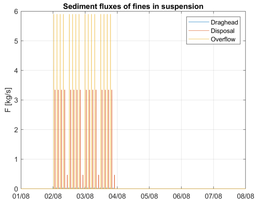
Figure Annex A-7 Timeseries of the implemented source of fines ( d_p < 63 \mu\text{m} ) [kg/s] as a result dredging trenches at trench section 1 for the power cables and disposing dredged material at a temporary disposal site 3.
