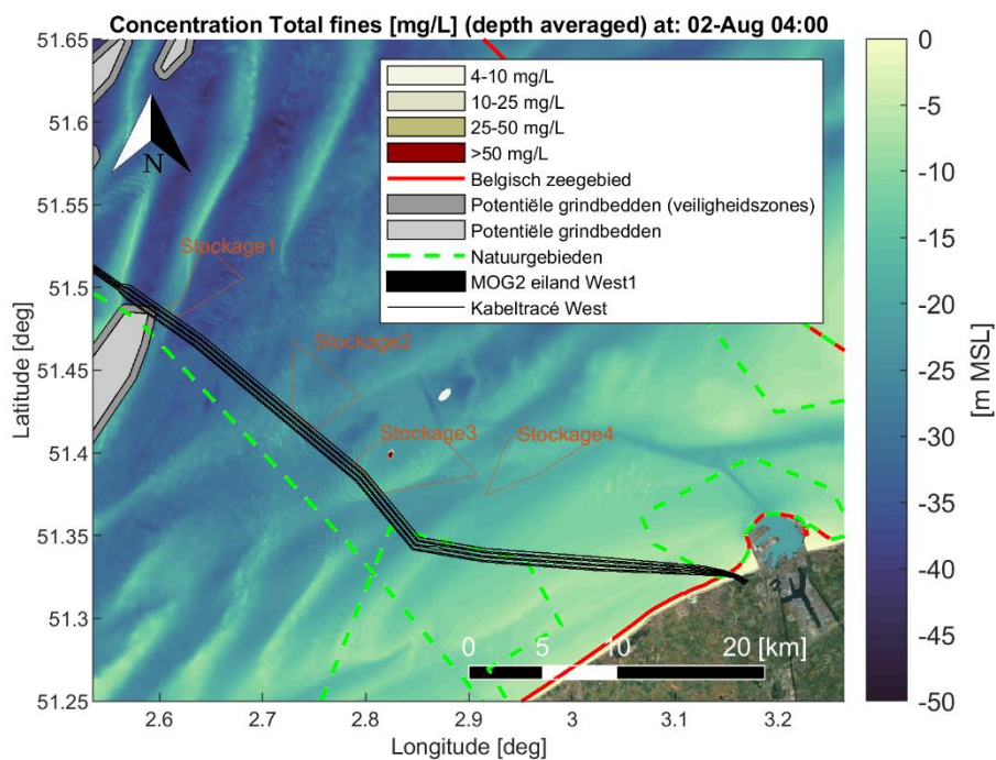
Figure Annex B-9 Map showing encountered depth averaged sediment concentration [mg/L] of fine material (< 250 [µm]) during a time instant of the simulation period. Scenario: Dredging cable trenches (trench1 section) and disposal at a temporary disposal site (Stockage3). Satellite background image credit: "OpenMapTiles.org".
