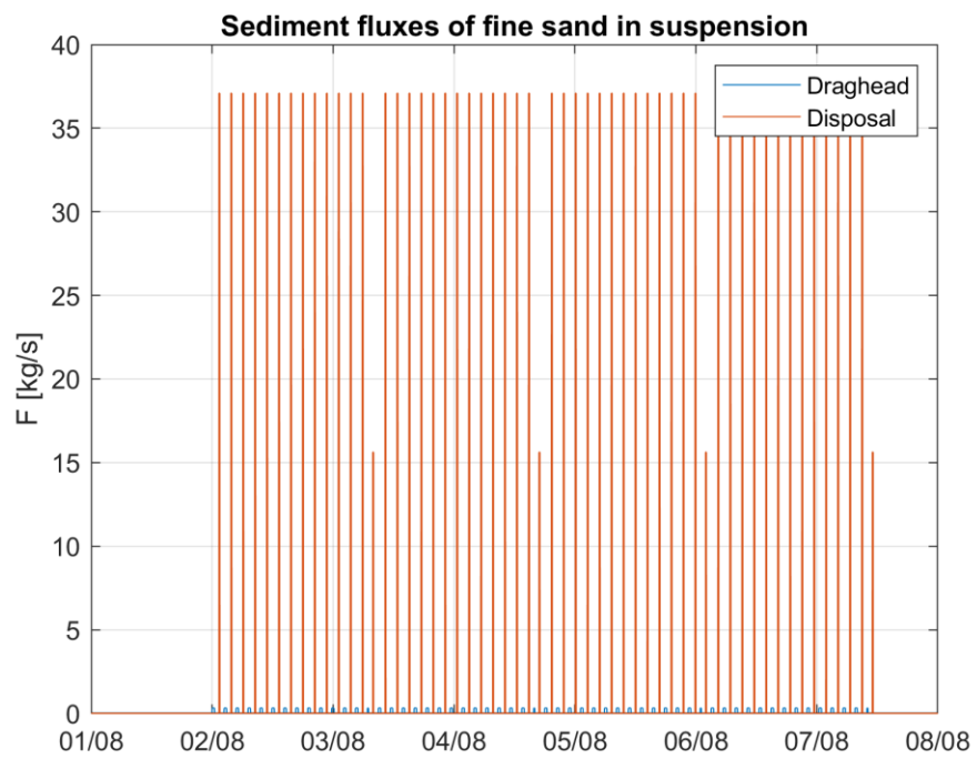
Figure Annex A-12 Time series of the implemented source of fine sand [kg/s] as a result dredging trenches at trench section 3 for the power cables and disposing dredged material at a temporary disposal site 3.
