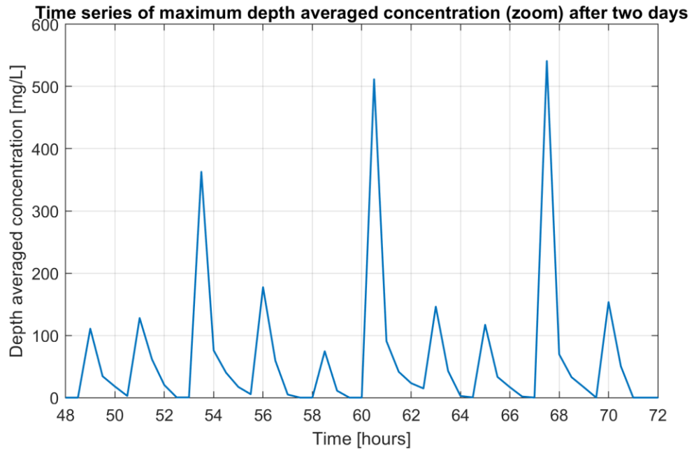
Figure 4-20 Time series of maximal sediment concentration [mg/L] of fine sediment at the temporary disposal site 3, using half-hourly model output. Zoom-in of 24 hours after two simulation days.
