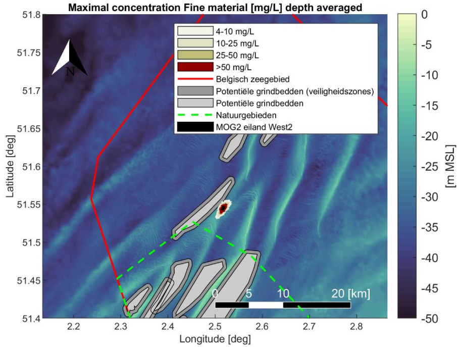
Figure 4-3 Maximal encountered depth averaged sediment concentration [mg/L] of fine material ( < 250 \mu m ) during the simulation period. Scenario: Plume generation while pre-dredging scour holes and ridges and disposing dredged material at the island location West 2.
