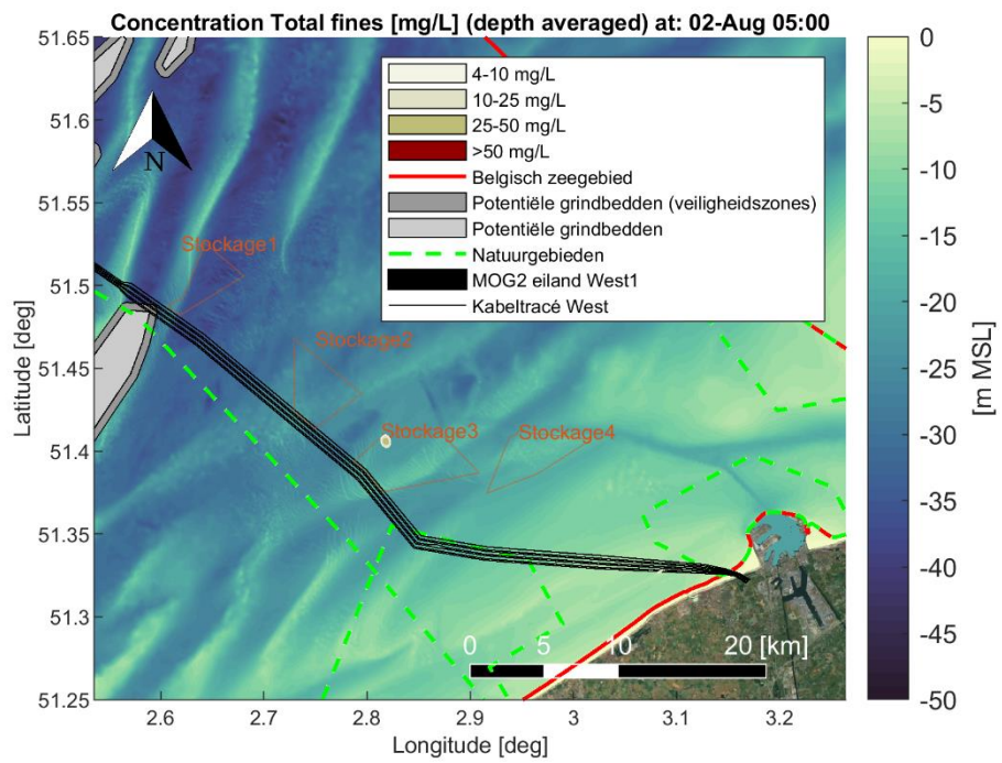
Figure Annex B-11 Map showing encountered depth averaged sediment concentration [mg/L] of fine material (< 250 [µm]) during a time instant of the simulation period. Scenario: Dredging cable trenches (trench1 section) and disposal at a temporary disposal site (Stockage3). Satellite background image credit: "OpenMapTiles.org".
