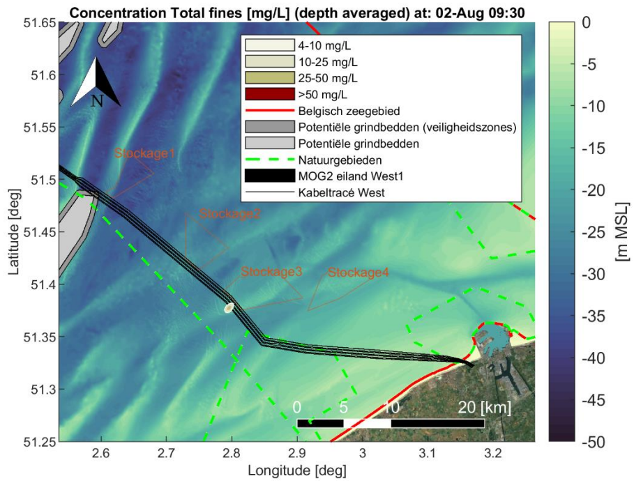
Figure Annex B-20 Map showing encountered depth averaged sediment concentration [mg/L] of fine material (< 250 [µm]) during a time instant of the simulation period. Scenario: Dredging cable trenches (trench1 section) and disposal at a temporary disposal site (Stockage3). Satellite background image credit: "OpenMapTiles.org".
