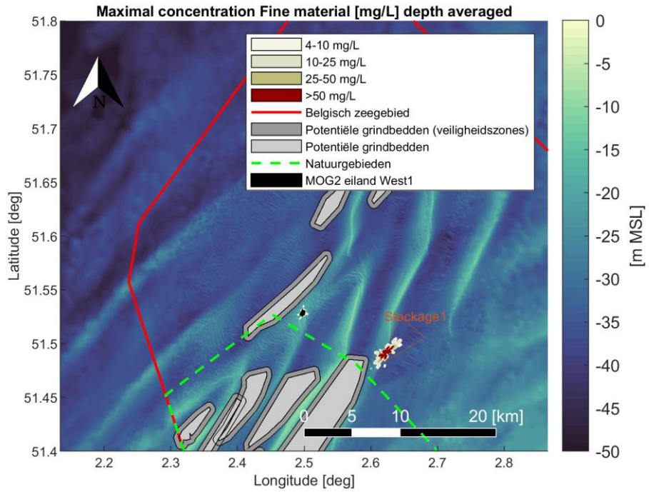
Figure 4-1 Maximal encountered depth averaged sediment concentration [mg/L] of fine material ( < 250 [\mu m] ) during the simulation period Scenario 1: levelling sand ridges and disposal at a temporary disposal site (island location West 1).
