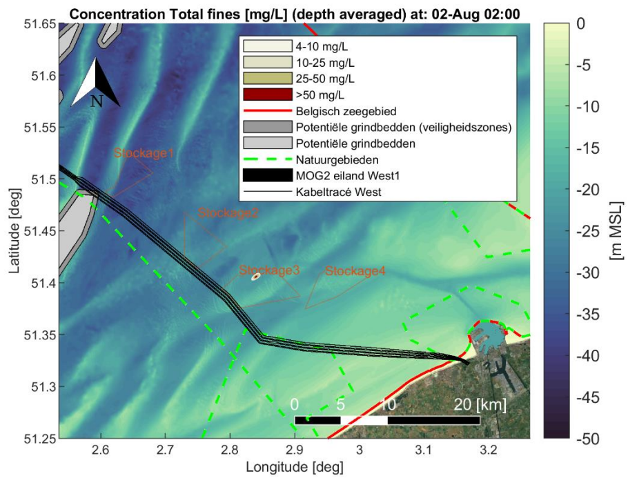
Figure Annex B-5 Map showing encountered depth averaged sediment concentration [mg/L] of fine material (< 250 [µm]) during a time instant of the simulation period. Scenario: Dredging cable trenches (trench1 section) and disposal at a temporary disposal site (Stockage3). Satellite background image credit: "OpenMapTiles.org".
