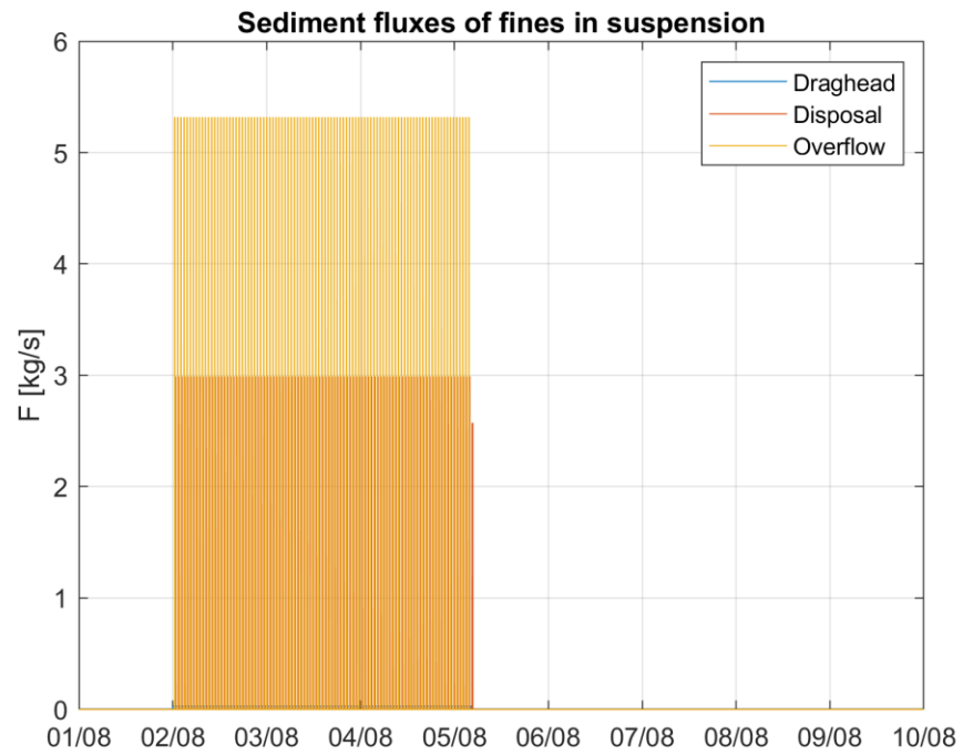
Figure 7-5 Time series of the implemented source of fines ( d_p < 63 \mu\text{m} ) [kg/s] as a result of pre-dredging scour holes and ridges and disposing dredged material at the island location at the Noord location.
