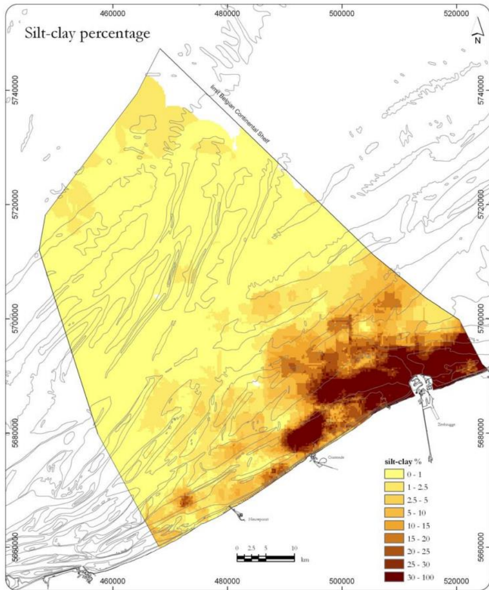
Figure 2-10 Map showing estimated silt-clay percentage in the Belgian sea zone (Van Lancker et al., 2007).
