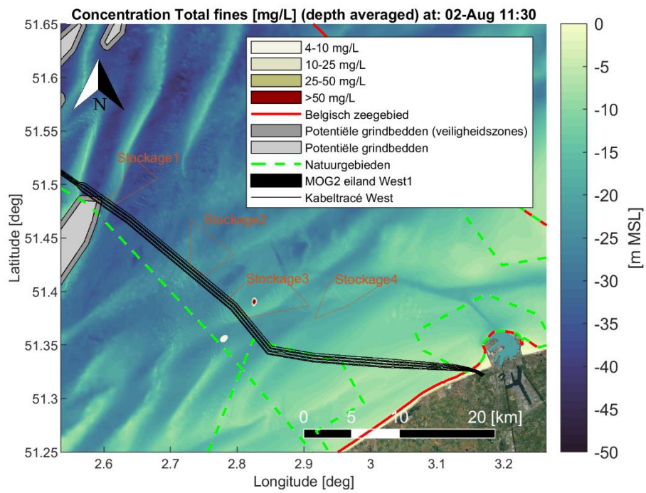
Figure Annex B-24 Map showing encountered depth averaged sediment concentration [mg/L] of fine material (< 250 [µm]) during a time instant of the simulation period. Scenario: Dredging cable trenches (trench1 section) and disposal at a temporary disposal site (Stockage3). Satellite background image credit: "OpenMapTiles.org".
