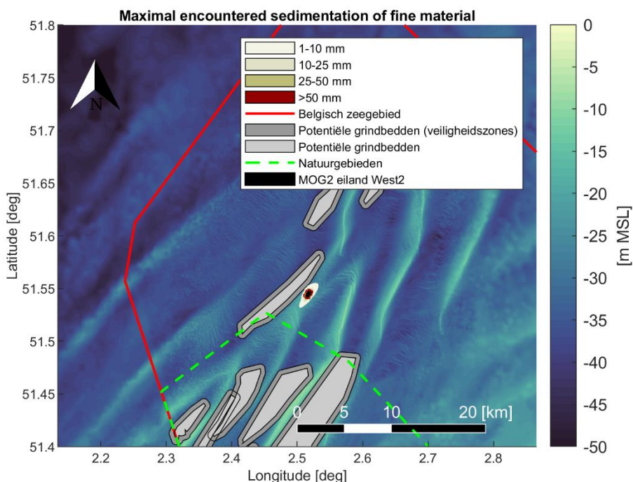
Figure 4-4 Maximal encountered sedimentation [mm] of fine material (< 250 \mu\text{m} ) during the simulation period. Scenario 2: pre-dredging scour holes and creation of sand plateau at the island location West2.
