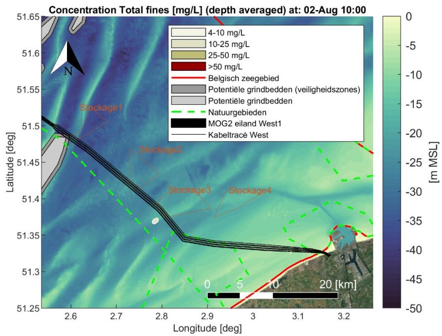
Figure Annex B-21 Map showing encountered depth averaged sediment concentration [mg/L] of fine material (< 250 \mu\text{m} ) during a time instant of the simulation period. Scenario: Dredging cable trenches (trench1 section) and disposal at a temporary disposal site (Stockage3). Satellite background image credit: "OpenMapTiles.org".
