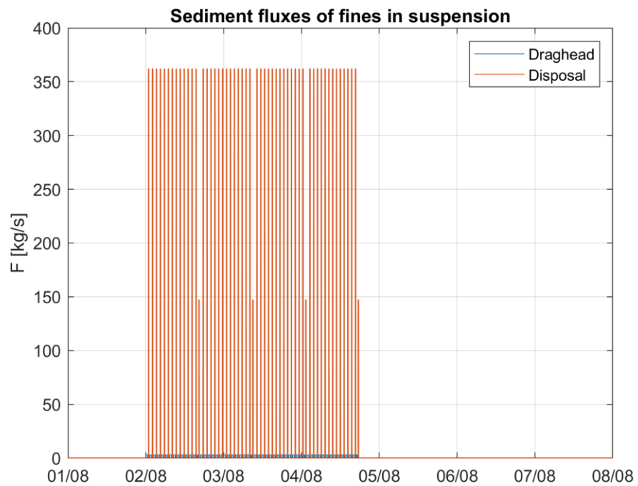
Figure Annex A-9 Timeseries of the implemented source of fines ( d_p < 63 \mu\text{m} ) [kg/s] as a result dredging trenches at trench section 2 for the power cables and disposing dredged material at a temporary disposal site 3.
