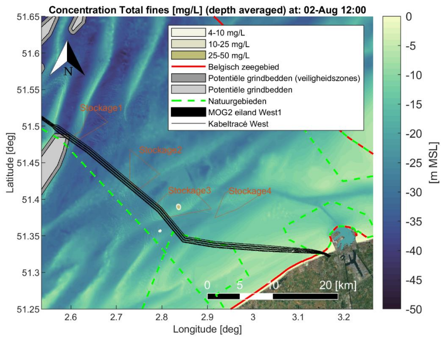
Figure Annex B-25 Map showing encountered depth averaged sediment concentration [mg/L] of fine material (< 250 [µm]) during a time instant of the simulation period. Scenario: Dredging cable trenches (trench1 section) and disposal at a temporary disposal site (Stockage3). Satellite background image credit: "OpenMapTiles.org".
