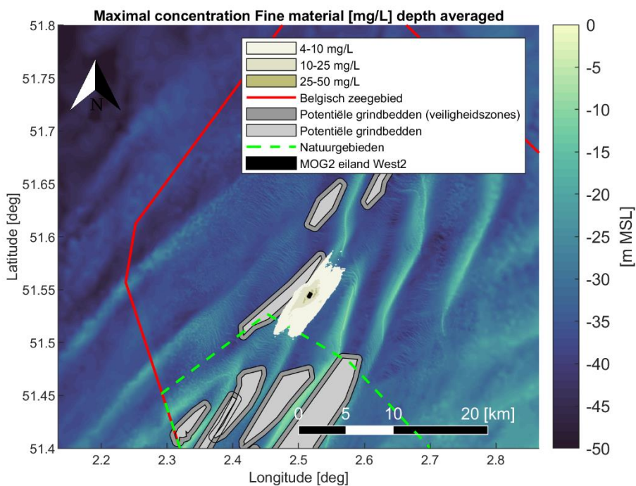
Figure 4-26 Maximal encountered depth averaged sediment concentration [mg/L] of fine material (< 250 [μm]) during the simulation period. Scenario: Plume generation and deposition as a result of natural erosion in one year time after West 2 island construction, after one year case.
