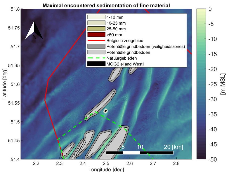
Figure 4-8 Maximal encountered sedimentation [mm] of fine material (< 250 [µm]) during the simulation period. Scenario 3: pre-dredging scour holes and filling the West 1 island ring.
