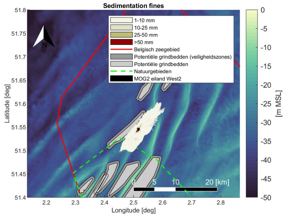
Figure 4-25 Maximal encountered sedimentation [mm] of fine material (< 250 [μm]) during the simulation period. Scenario: Plume generation and deposition as a result of natural erosion in one year time after West 2 island construction, after one year case..
