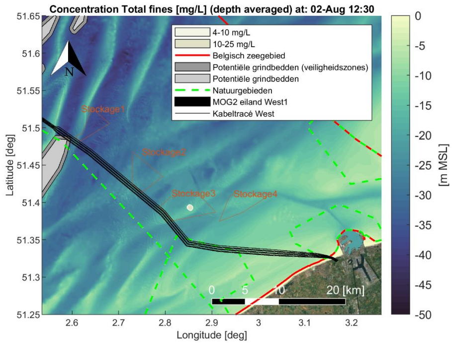
Figure Annex B-26 Map showing encountered depth averaged sediment concentration [mg/L] of fine material (< 250 [µm]) during a time instant of the simulation period. Scenario: Dredging cable trenches (trench1 section) and disposal at a temporary disposal site (Stockage3). Satellite background image credit: "OpenMapTiles.org".
