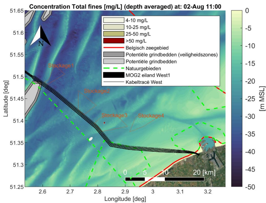
Figure Annex B-23 Map showing encountered depth averaged sediment concentration [mg/L] of fine material (< 250 \mu\text{m} ) during a time instant of the simulation period. Scenario: Dredging cable trenches (trench1 section) and disposal at a temporary disposal site (Stockage3). Satellite background image credit: "OpenMapTiles.org".
