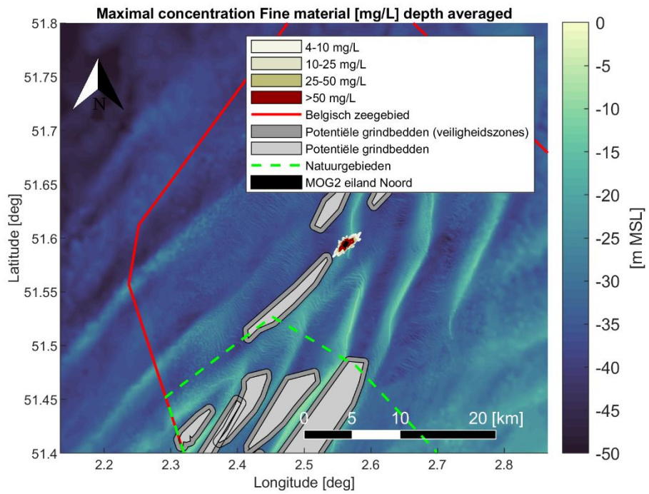
Figure 4-5 Maximal encountered depth averaged sediment concentration [mg/L] of fine material ( < 250 [\mu m] ) during the simulation period. Scenario 2: pre-dredging scour holes and creation of sand plateau at the island location Noord.
