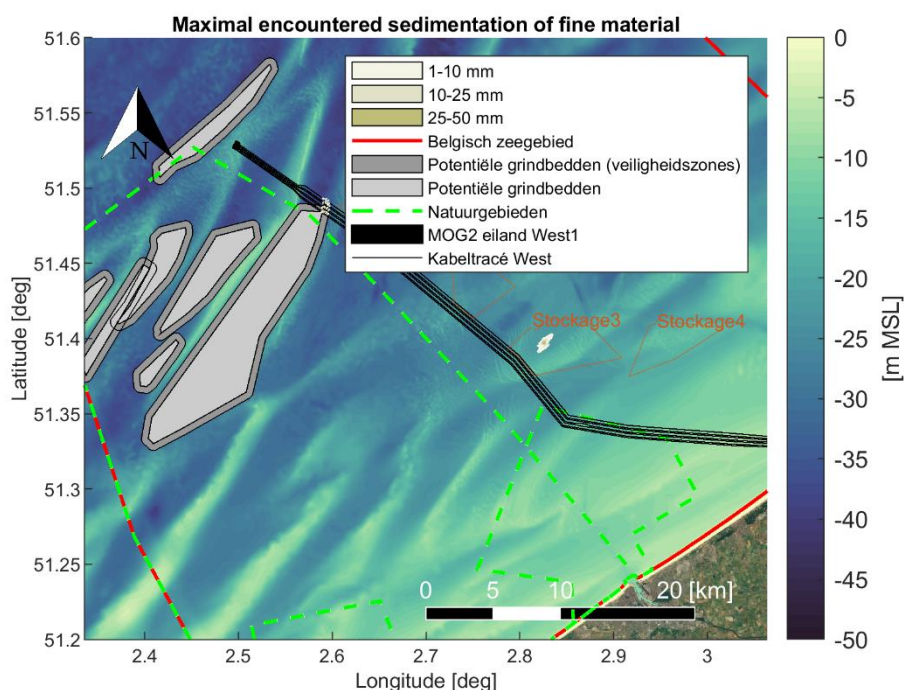
Figure 4-14 Maximal sedimentation [mm] of fine material ( < 250 \mu\text{m} ) during the simulation period. Scenario: Dredging cable trenches (trench1 section) and disposal at a temporary disposal site (Stockage3). Satellite background image credit: "OpenMapTiles.org".
