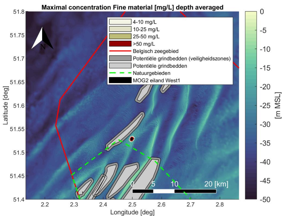
Figure 4-7 Maximal encountered depth averaged sediment concentration [mg/L] of fine material ( < 250 [\mu m] ) during the simulation period. Scenario 3: pre-dredging scour holes and filling the West 1 island ring.
