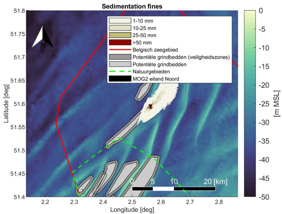
Figure 4-29 Maximal encountered sedimentation [mm] of fine material (< 250 [μm]) during the simulation period. Scenario: Plume generation and deposition as a result of natural erosion in one year time after Noord island construction, after one year case.
