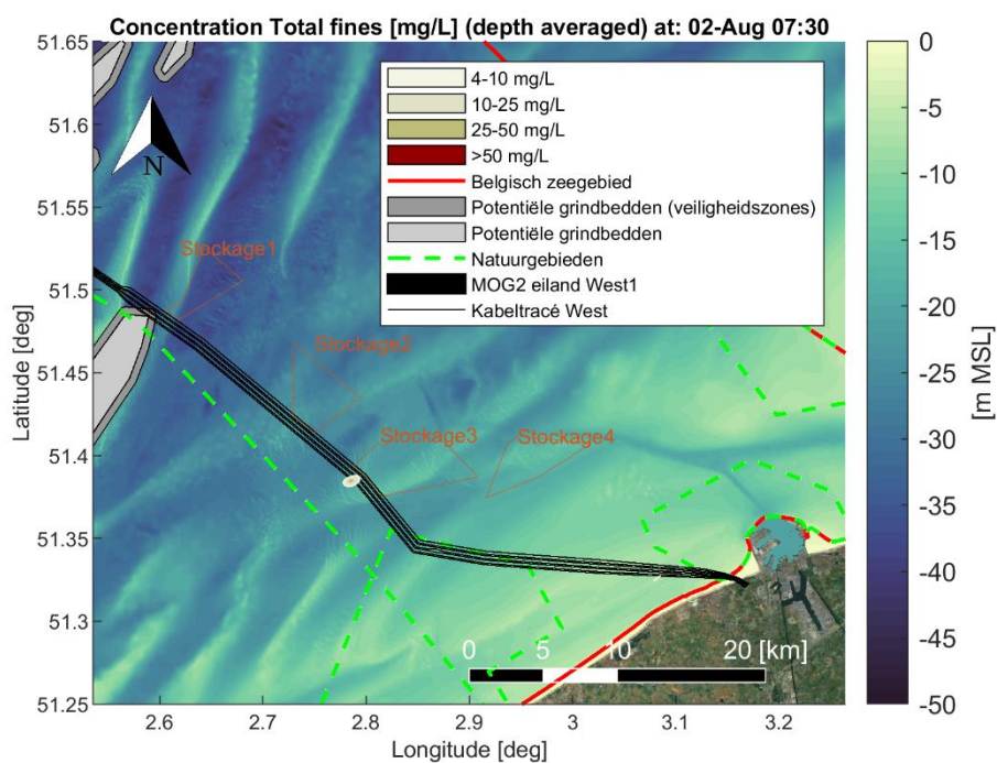
Figure Annex B-16 Map showing encountered depth averaged sediment concentration [mg/L] of fine material (< 250 [µm]) during a time instant of the simulation period. Scenario: Dredging cable trenches (trench1 section) and disposal at a temporary disposal site (Stockage3). Satellite background image credit: "OpenMapTiles.org".
