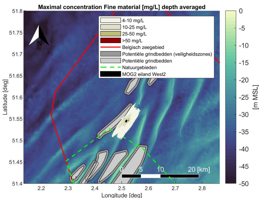
Figure 4-28 Maximal encountered depth averaged sediment concentration [mg/L] of fine material (< 250 [µm]) during the simulation period. Scenario: Plume generation and deposition as a result of natural erosion in one year time after West 2 island construction, after four year case.
