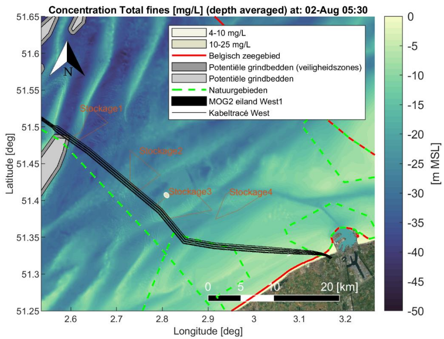
Figure Annex B-12 Map showing encountered depth averaged sediment concentration [mg/L] of fine material (< 250 [μm]) during a time instant of the simulation period. Scenario: Dredging cable trenches (trench1 section) and disposal at a temporary disposal site (Stockage3). Satellite background image credit: "OpenMapTiles.org".
