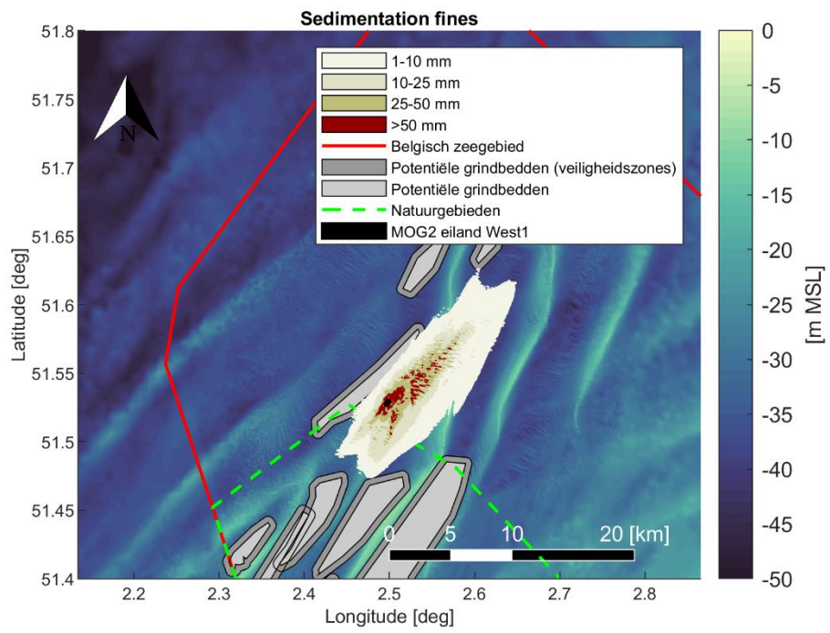
Figure 4-34 Maximal encountered sedimentation [mm] of fine material (< 250 [μm]) during the simulation period. Scenario: Plume generation and deposition as a result of natural erosion in one year time after West 1 island construction, after one year case without pre-scour design.
