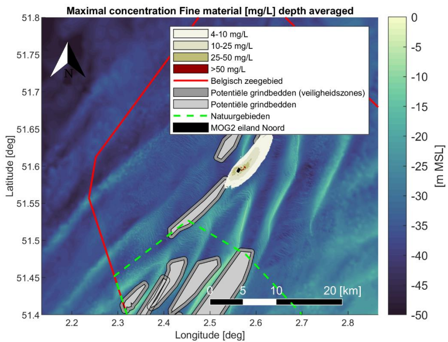
Figure 4-30 Maximal encountered depth averaged sediment concentration [mg/L] of fine material (< 250 [μm]) during the simulation period. Scenario: Plume generation and deposition as a result of natural erosion in one year time after Noord island construction, after one year case.
