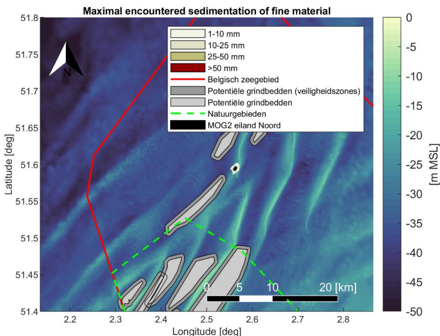
Figure 4-12 Maximal encountered sedimentation [mm] of fine material (< 250 [µm]) during the simulation period. Scenario 3: pre-dredging scour holes and filling the Noord island ring.
