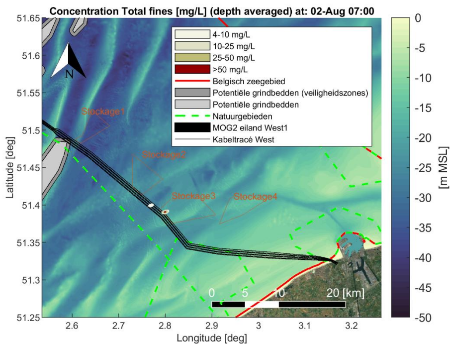
Figure Annex B-15 Map showing encountered depth averaged sediment concentration [mg/L] of fine material (< 250 [µm]) during a time instant of the simulation period. Scenario: Dredging cable trenches (trench1 section) and disposal at a temporary disposal site (Stockage3). Satellite background image credit: "OpenMapTiles.org".
