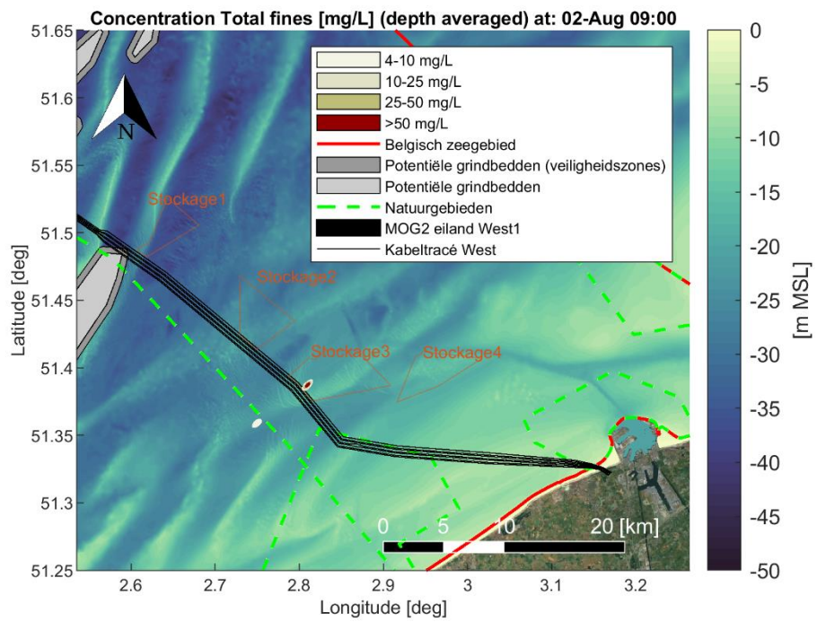
Figure Annex B-19 Map showing encountered depth averaged sediment concentration [mg/L] of fine material (< 250 [µm]) during a time instant of the simulation period. Scenario: Dredging cable trenches (trench1 section) and disposal at a temporary disposal site (Stockage3). Satellite background image credit: "OpenMapTiles.org".
