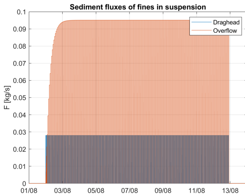
Figure Annex A-5 Time series of the implemented source of fines ( d_p < 63 \mu\text{m} ) [ \text{kg/s} ] as a result of pre-dredging scour holes and ridges and filling the island ring with dredged sand through pipes, leading to overflow from the island ring at the Noord location.
