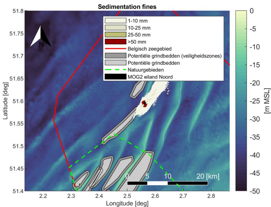
Figure 4-31 Maximal encountered sedimentation [mm] of fine material (< 250 [μm]) during the simulation period. Scenario: Plume generation and deposition as a result of natural erosion in one year time after Noord island construction, after four year case.
