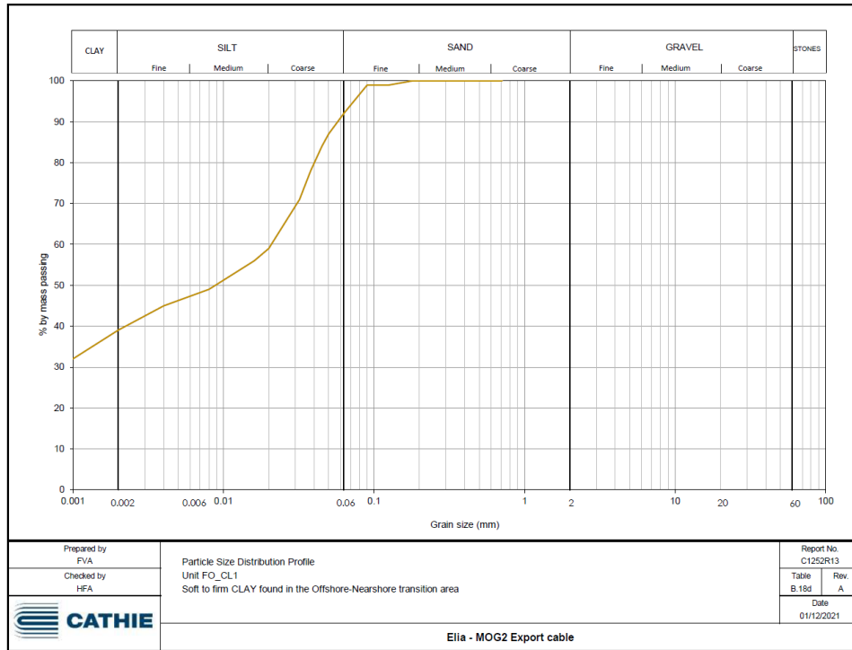
Figure 2-11 Particle size distribution profile of unit FO_CL1 (soft to firm clay found in the offshore-nearshore transition zone), adapted from Cathie draft report (2021).
