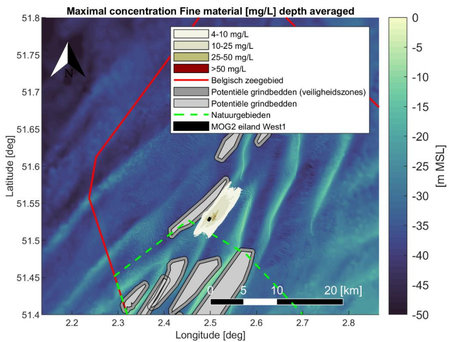
Figure 4-24 Maximal depth averaged sediment concentration [mg/L] of fine material (< 250 [µm]) during the simulation period. Scenario: : Plume generation and deposition as a result of natural erosion in one year time after West 1 island construction, after four year case..
