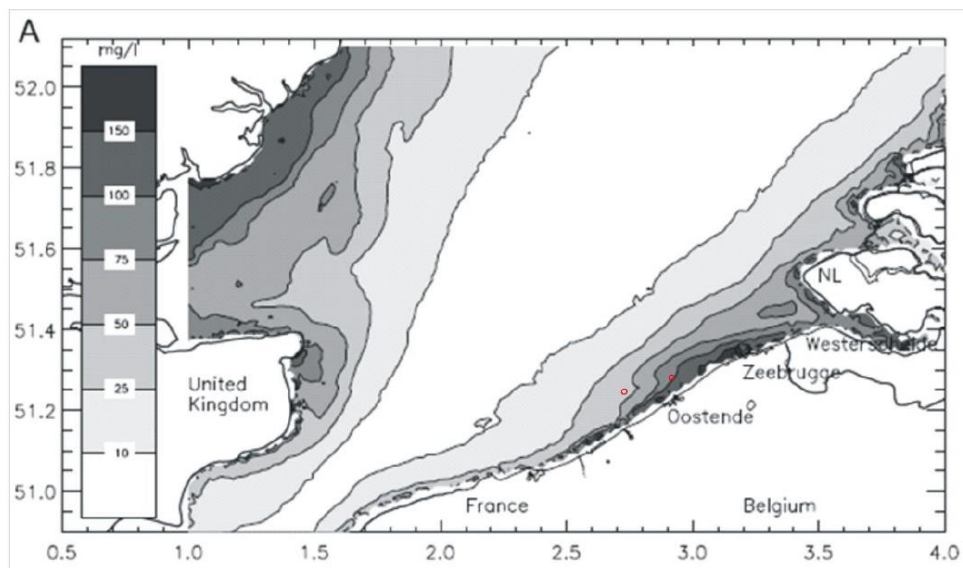
Figure 2-16 Yearly average of depth averaged SPM (Suspended Particulate Matter) concentrations [mg/L] in the southern part of the North sea estimated by Fettweis et al. (2010) .
