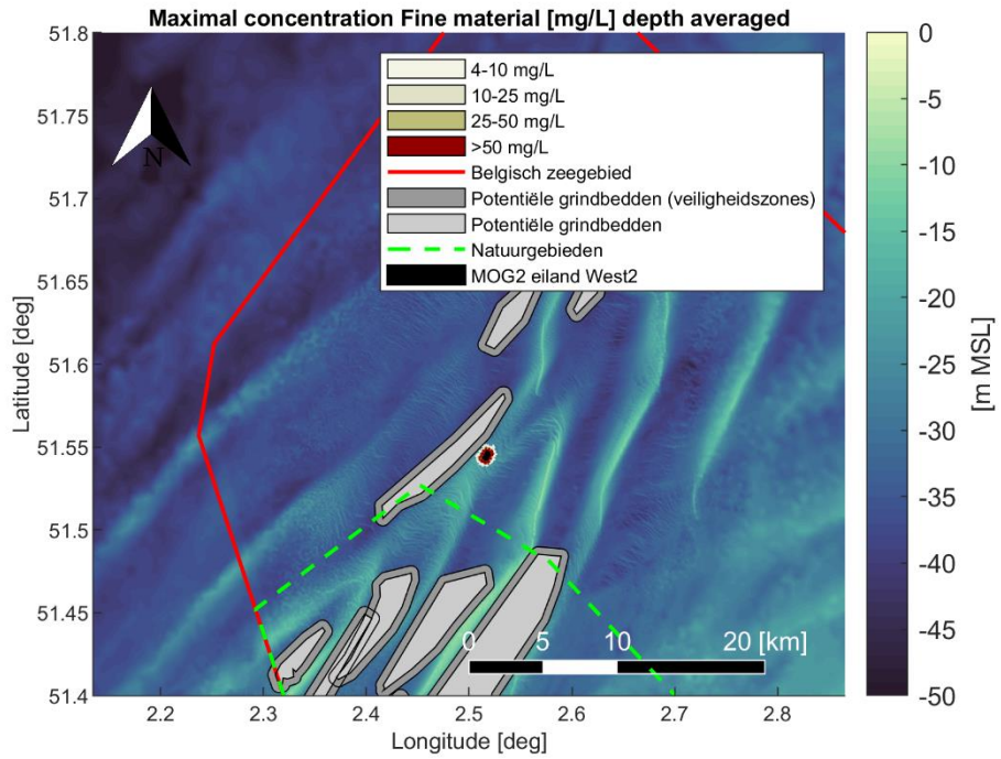
Figure 4-9 Maximal encountered depth averaged sediment concentration [mg/L] of fine material ( < 250 [\mu m] ) during the simulation period. Scenario 3: pre-dredging scour holes and filling the West 2 island ring.
