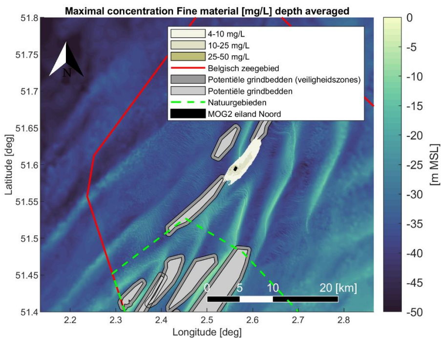
Figure 4-32 Maximal encountered depth averaged sediment concentration [mg/L] of fine material (< 250 [μm]) during the simulation period. Scenario: Plume generation and deposition as a result of natural erosion in one year time after Noord island construction, after four year case.
