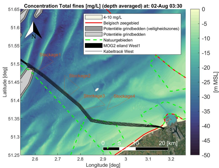
Figure Annex B-8 Map showing encountered depth averaged sediment concentration [mg/L] of fine material (< 250 [μm]) during a time instant of the simulation period. Scenario: Dredging cable trenches (trench1 section) and disposal at a temporary disposal site (Stockage3). Satellite background image credit: "OpenMapTiles.org".
