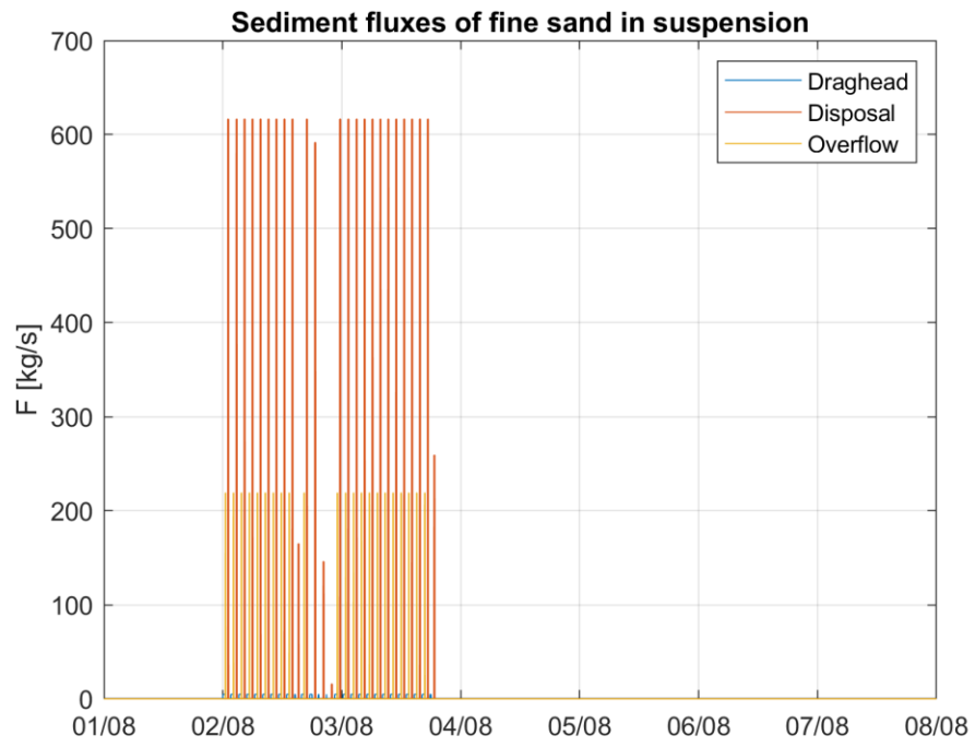
Figure 7-2 Time series of the implemented source of fine sand [kg/s] as a result of dredging works related to the levelling of sand ridge crests at the West 1 location.
