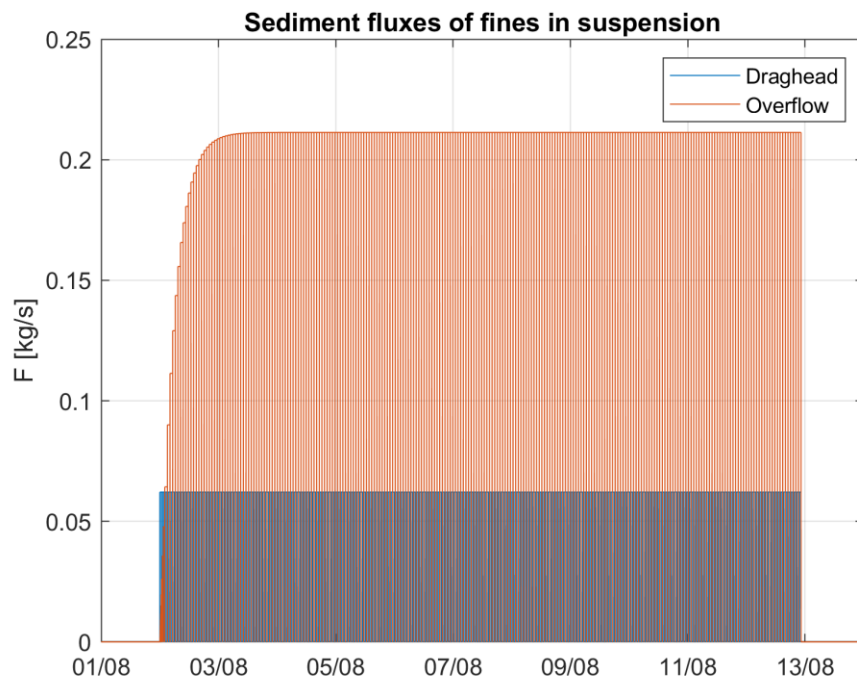
Figure Annex A-3 Time series of the implemented source of fines ( d_p < 63 \mu\text{m} ) [ \text{kg/s} ] as a result of pre-dredging scour holes and ridges and filling the island ring with dredged sand through pipes, leading to overflow from the island ring at the West 2 location.
